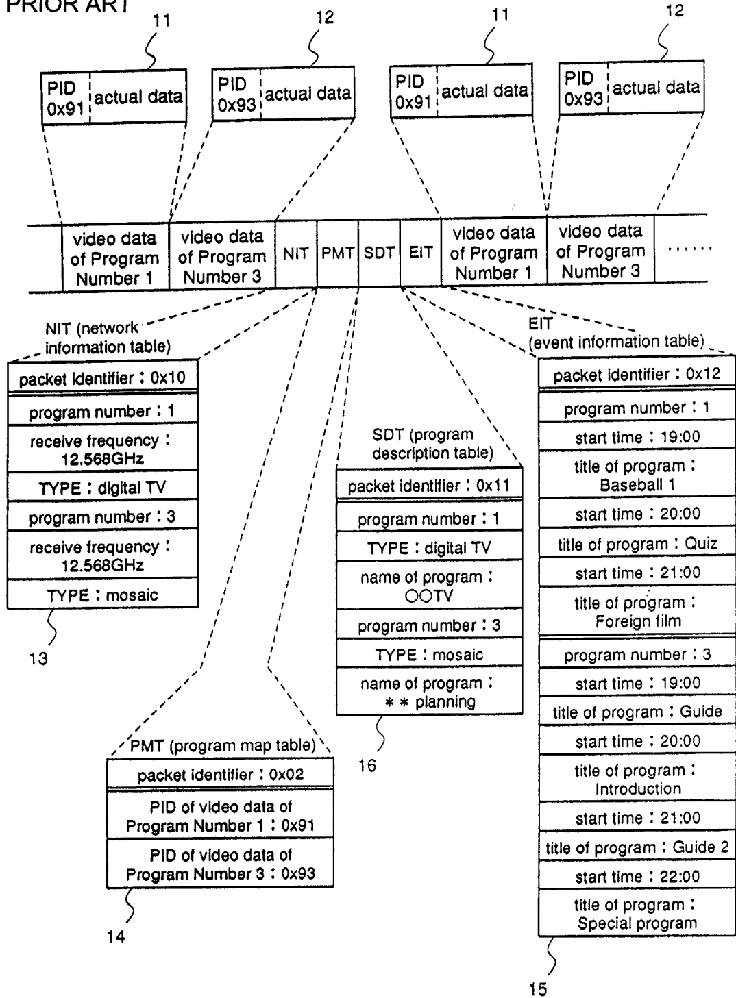
Fig.32 PRIOR ART
