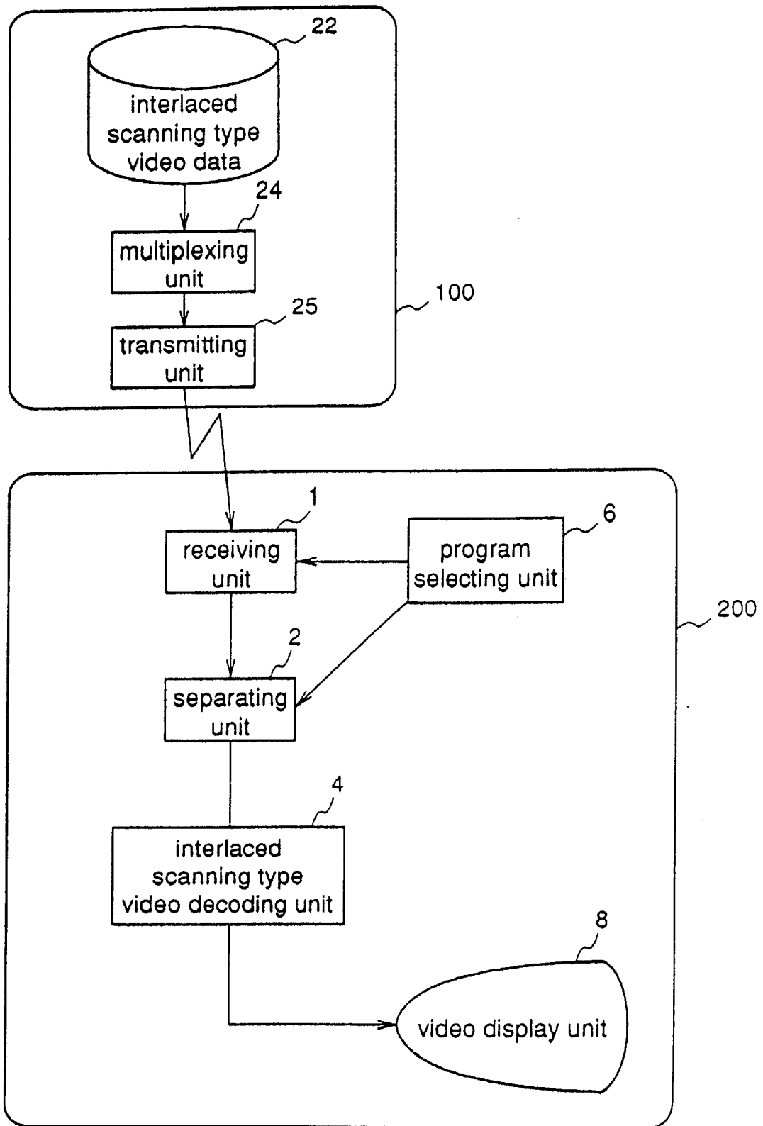
Fig.30 PRIOR ART
