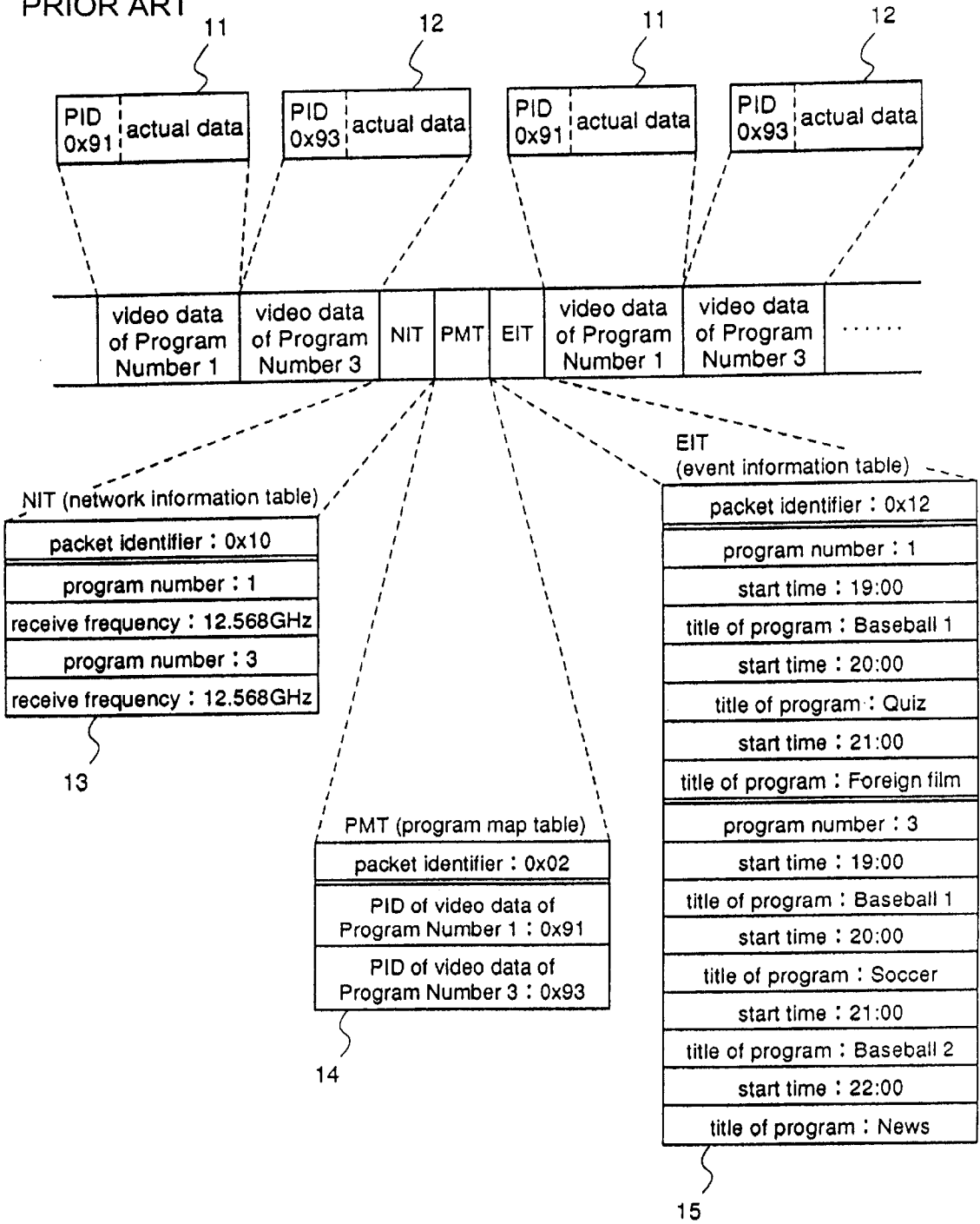
Fig.29 PRIOR ART
