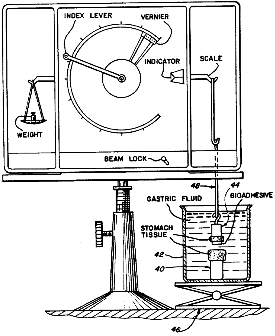
MODIFIED SURFACE TENSIO METER
