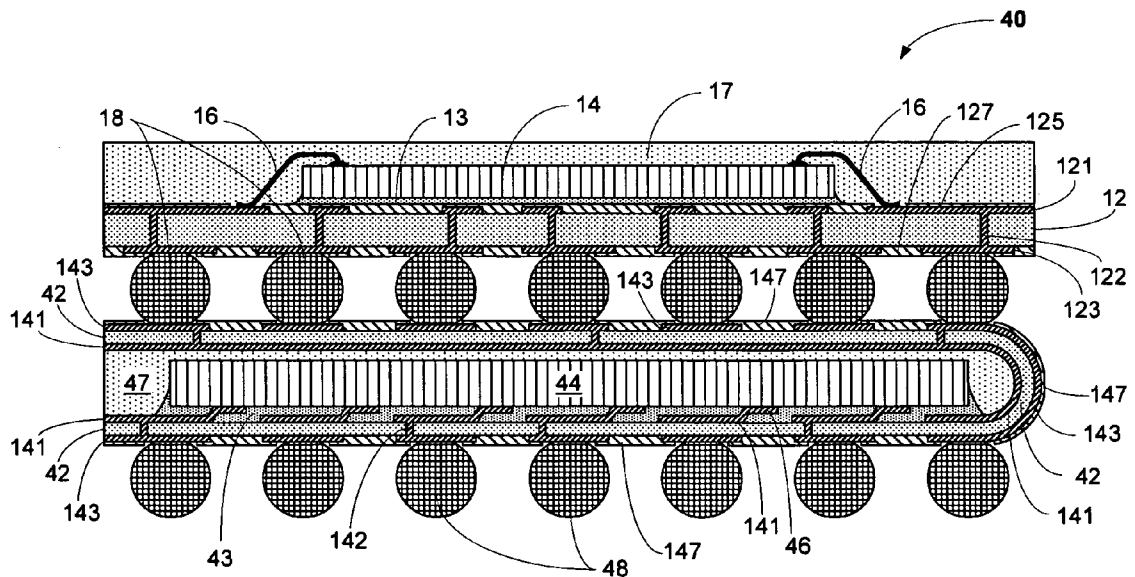
Fig. 4 PRIOR ART
