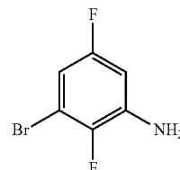
3-bromo-2,5-difluoroaniline
