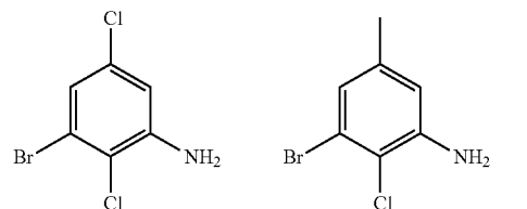
3-bromo-2,5-dichloroaniline 3-bromo-2-chloro-5-methylaniline
