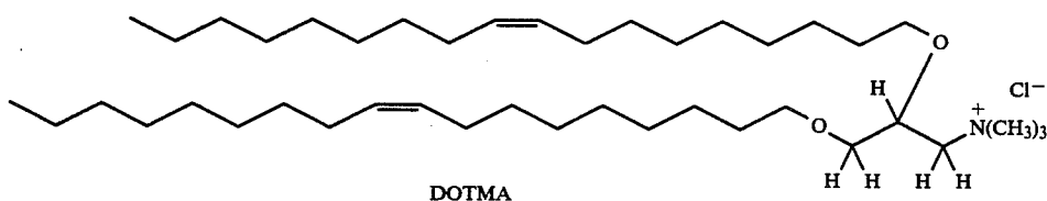
FIG. 1: Synthesis of DOTMA
