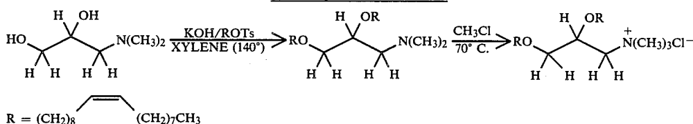
FIG. 1: Synthesis of DOTMA
