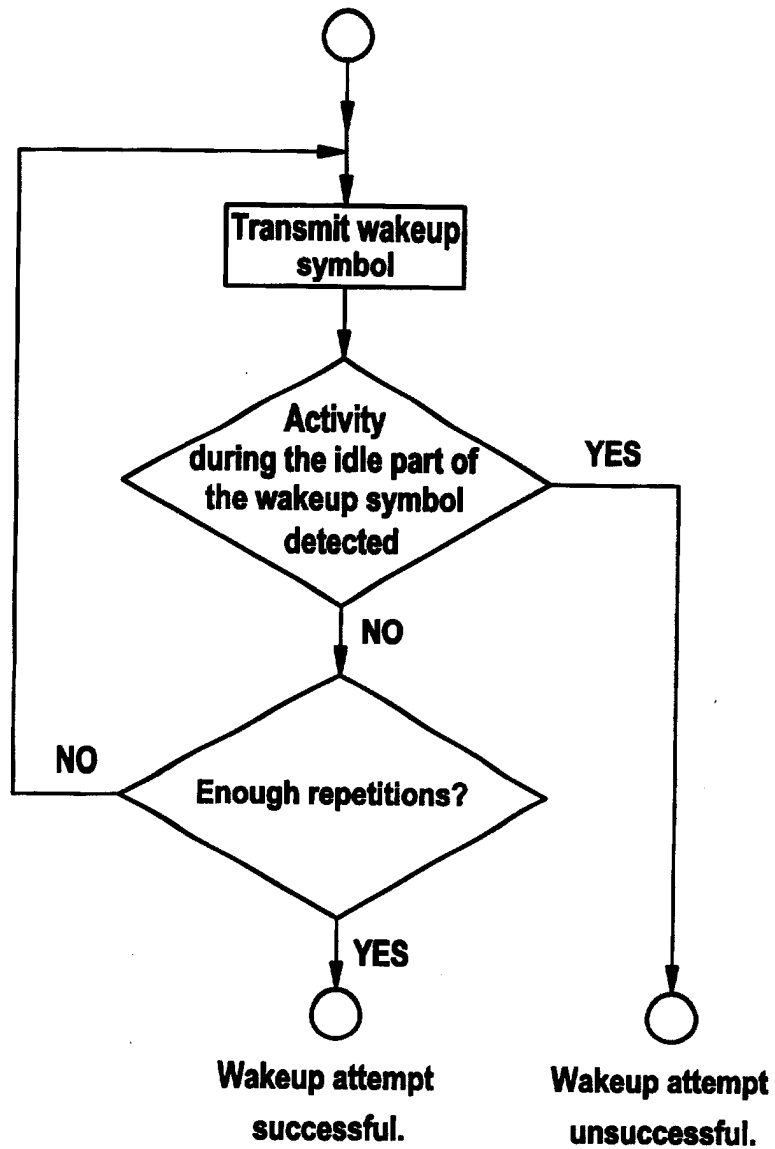
Wakeup pattern transmission
