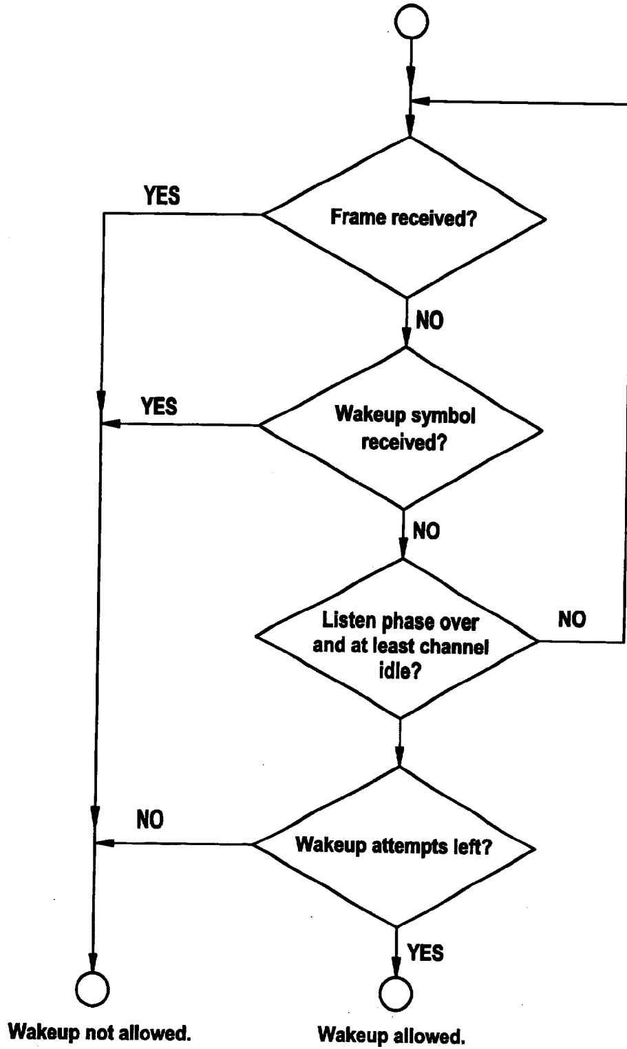
Wakeup channel monitoring
