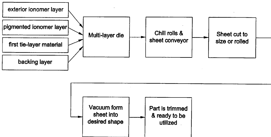
An embodiment of a co-extrusion and vacuum forming (thermoforming) process.
