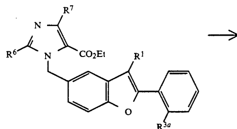
Equation 4
