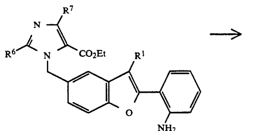
Equation 3
