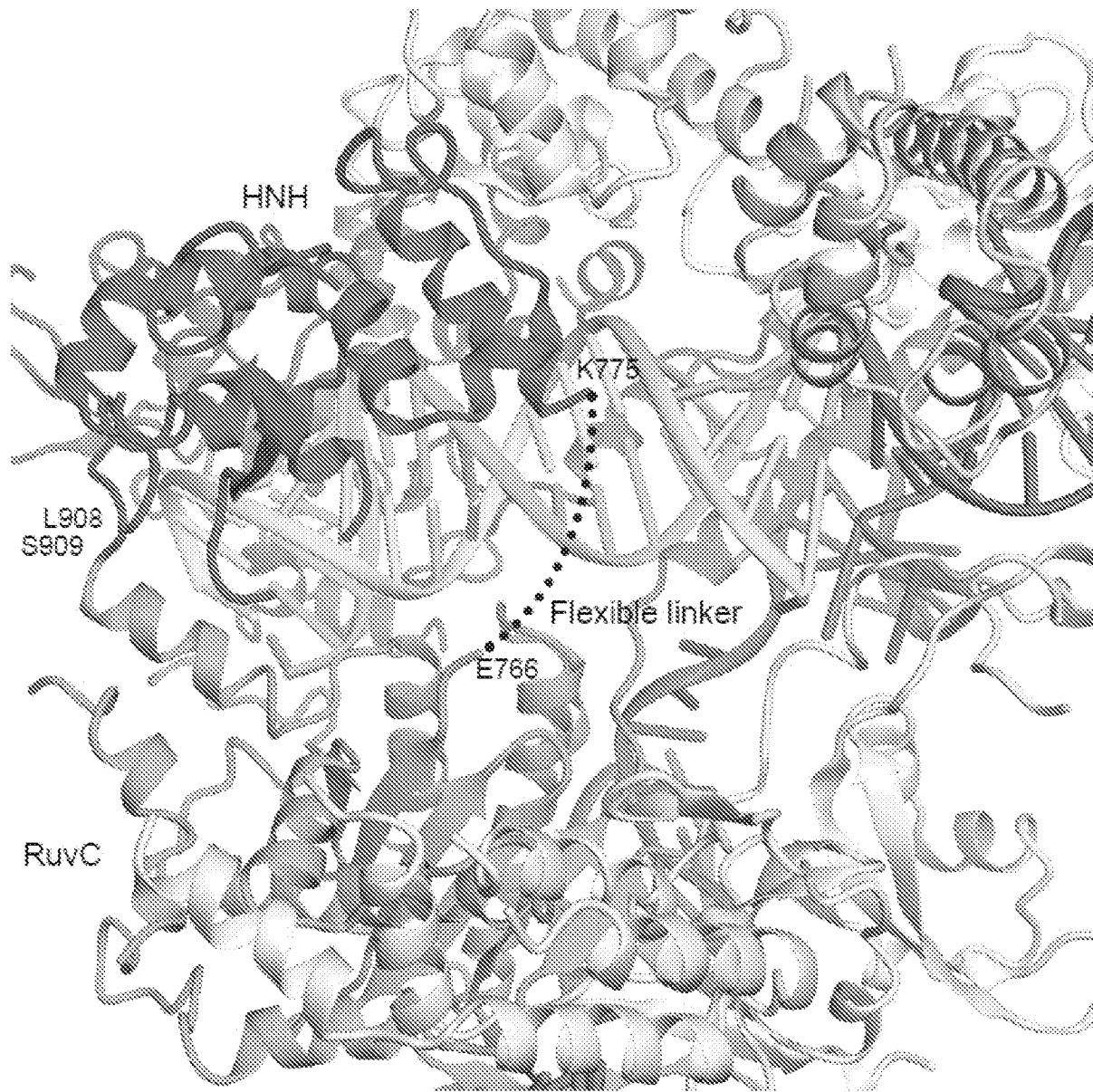
RuvC (E766)-linker-Effector-linker-RuvC (S909)
