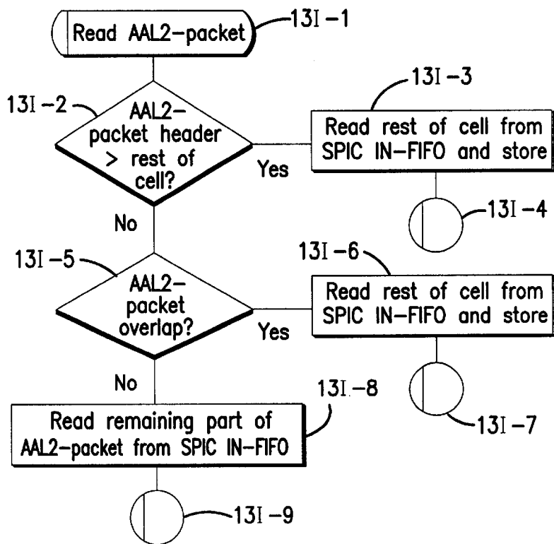
FIG. 13I READ AAL2 PACKET
