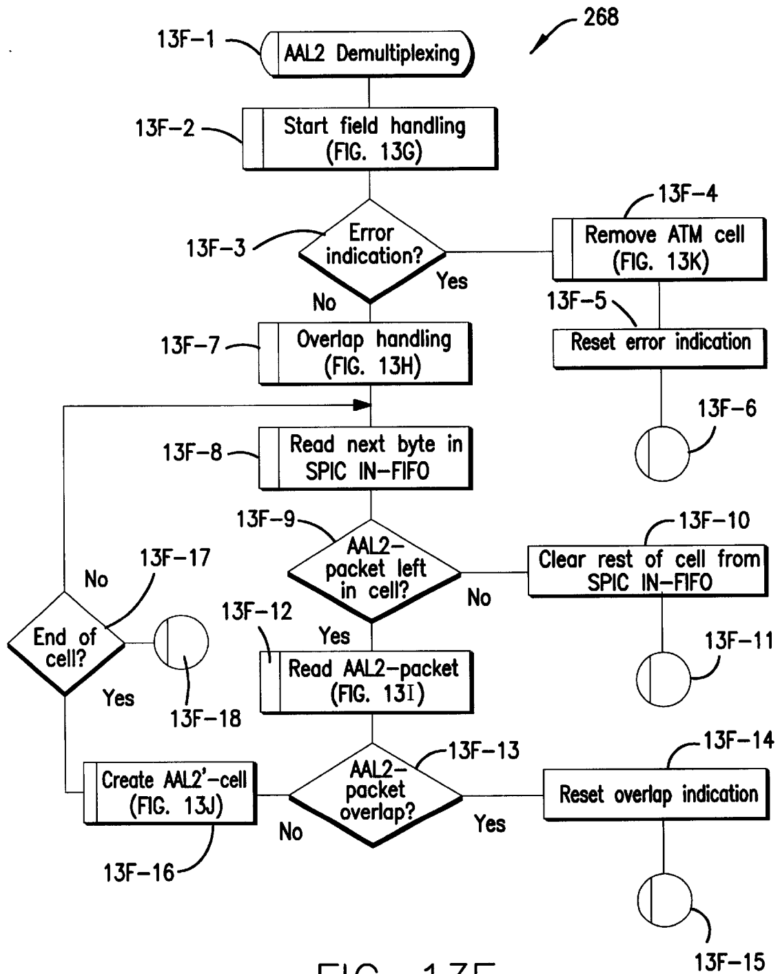
FIG. 13F AAL2 DEMULPLEXING
