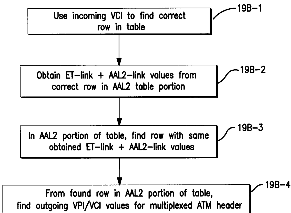
FIG. 19B COMBINED TABLE LOOK-UP PROCEDURE FOR MULTIPLEXING
