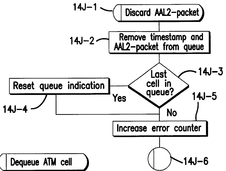
FIG. 14J DISCARD AAL2 PACKET FUNCTION
