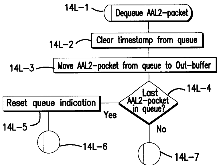
FIG. 14L DEQUEUE AAL2 PACKET FUNCTION
