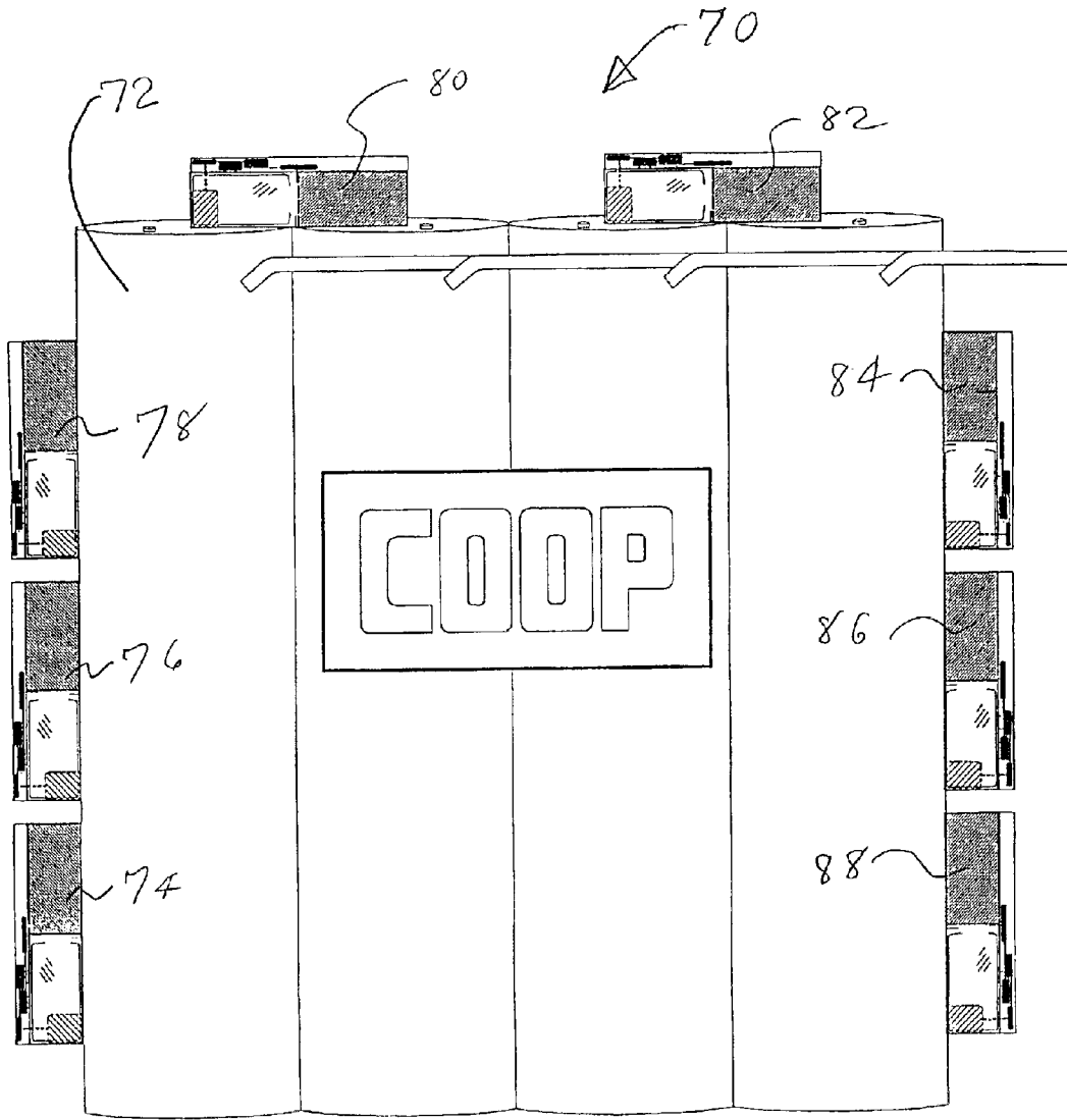
GRAIN ELEVATOR FIG. 8
