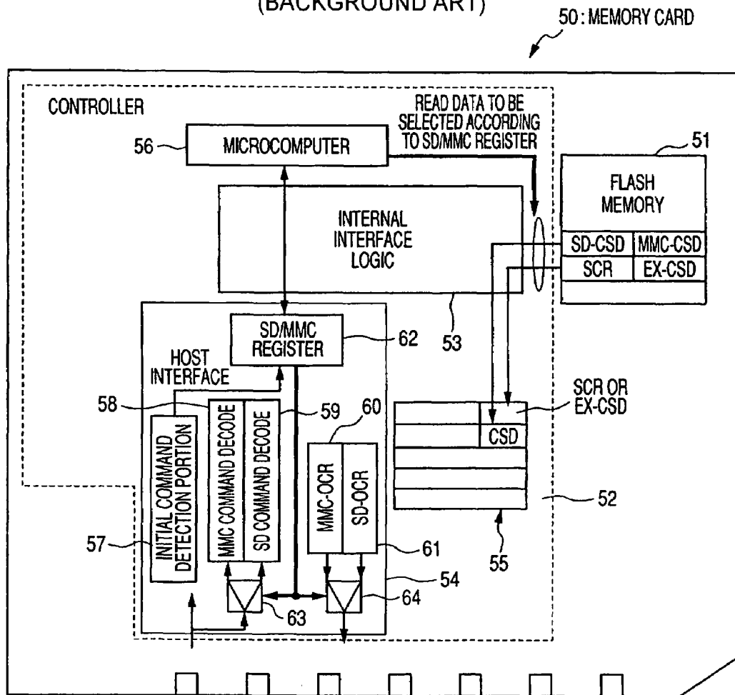
FIG. 12 (BACKGROUND ART)
