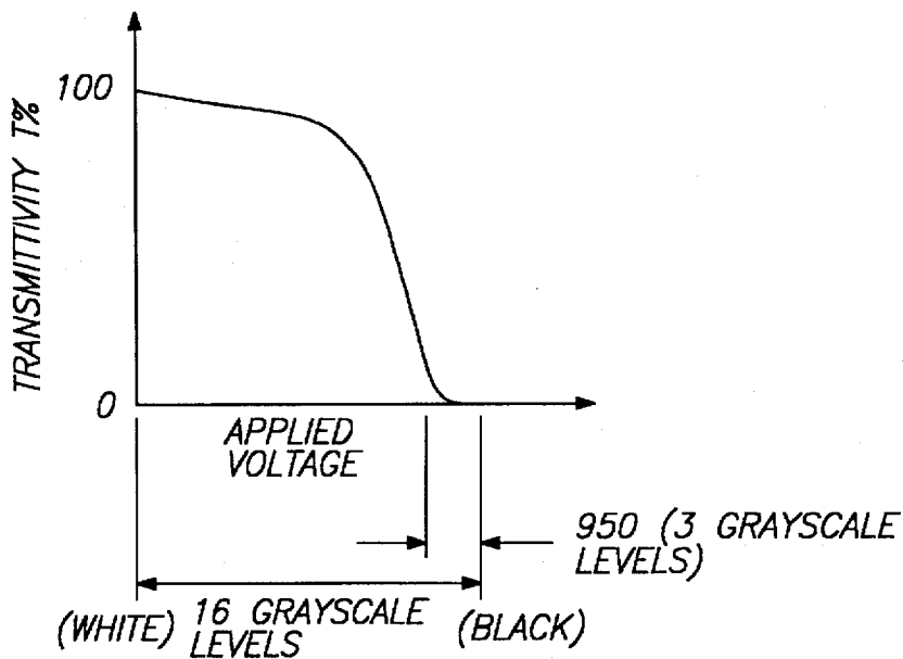
FIG.-28 (PRIOR ART)
