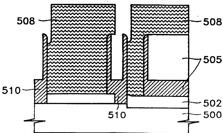
FIG. 1C(PRIOR ART)
