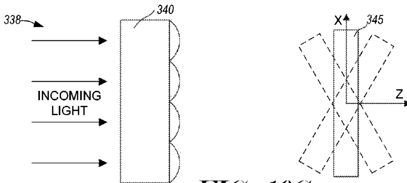
FIG. 10C (TOP VIEW)
