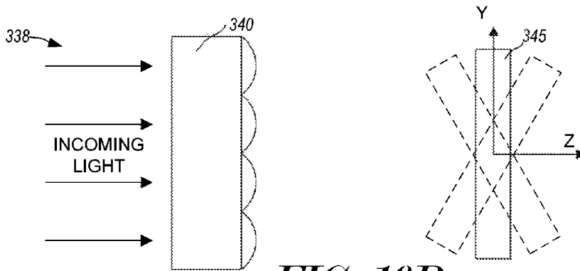
FIG. 10B (SIDE VIEW)
