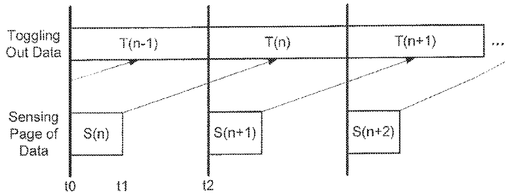
Conventional Read Caching
