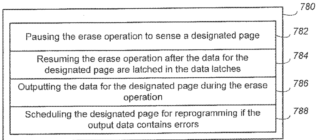
Caching Read Scrubbing Operation During Erase Operation
