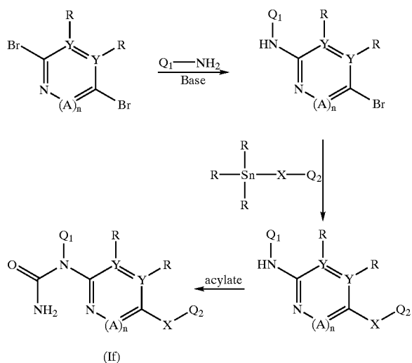
Scheme 7
