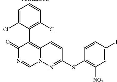
compound 34
