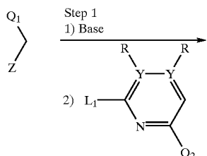
SCHEME 4
