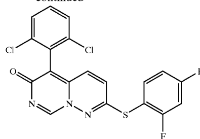
compound 53
