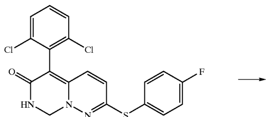
compound 103
