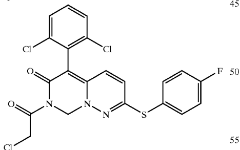
compound 103
