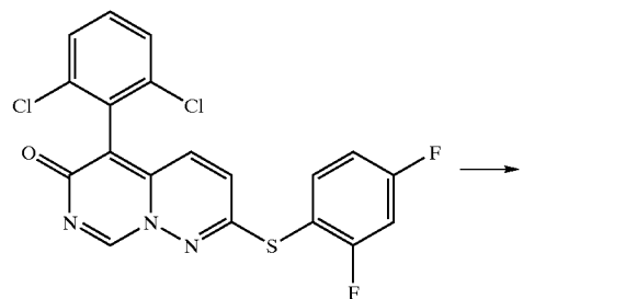
compound 53
