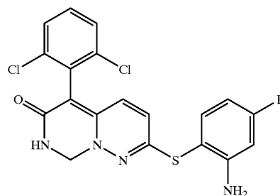
compound 117
