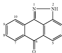
2H-Dibenzo[cd,g]indazol-6-one
