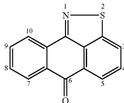
Anthra[9,1-cd]isothiazol-6-one
