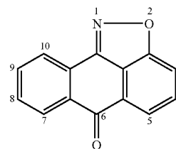
2-Oxa-1-aza-aceanthrylen-6-one
