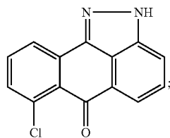
7-Chloro-2H-dibenzo[cd,g] indazol-6-one
