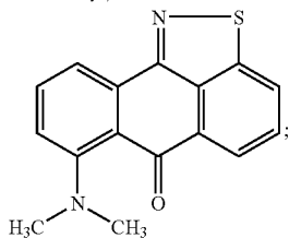
7-Dimethylamino-anthra[9,1-cd]isothiazol-6-one
