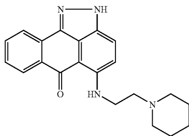
5-(2-Piperidin-1-yl-ethylamino)-2H- dibenzo[cd,g]indazole-6-one
