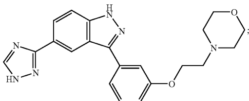
3-[3-(2-Morpholin-4-yl-ethoxy)-phenyl]-5-(1H-[1,2,4]triazol-3-yl)-1H-indazole
