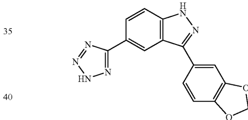
3-Benzo[1,3]dioxol-5-yl-5-(2H-tetrazol-5-yl)-1H-indazole
