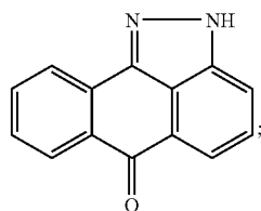
2H-Dibenzo[cd,g] indazol-6-one
