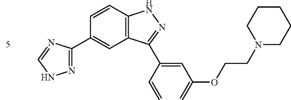
3-[3-(2-Piperidin-1-yl-ethoxy)-phenyl]-5-(1H-[1,2,4]triazol-3-yl)-1H-indazole
