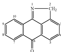
2H-Dibenzo[cd,g]indol-6-one
