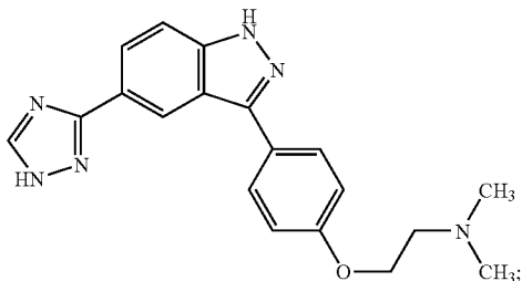
Dimethyl-(2-(4-[5-(1H-[1,2,4]triazol-3-yl)-1H-indazol-3-yl]-phenoxy)-ethyl)-amine
