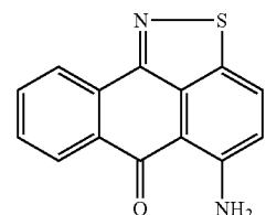
5-Amino-anthra[9,1- cd]isothiazol-6-one
