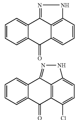
5-Chloroanthra[1,9cd]pyrazol-6(2H)-one
