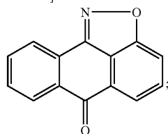
2-Oxa-1-aza-aceanthrylen-6-one
