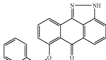
7-Benzyloxy-2H-dibenzo[cd,g]indazol- 6-one
