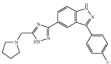
3-(4-Fluoro-phenyl)-5-(5-pyrrolidin-1-ylmethyl-1H-[1,2,4]triazol-3-yl)-1H-indazole
