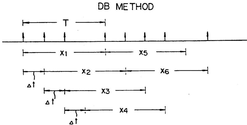
Fig. 31 PRIOR ART
