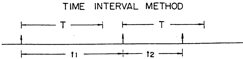
Fig. 30 PRIOR ART
