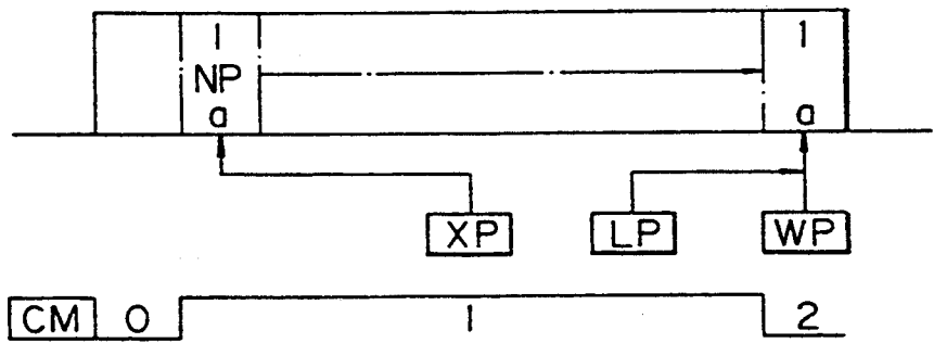
Fig. 14C (SHIFT)
