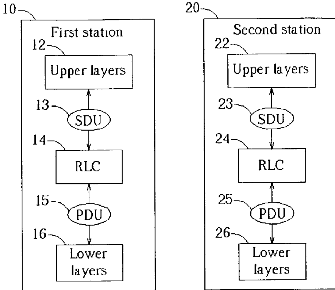
Fig. 1 Prior art
