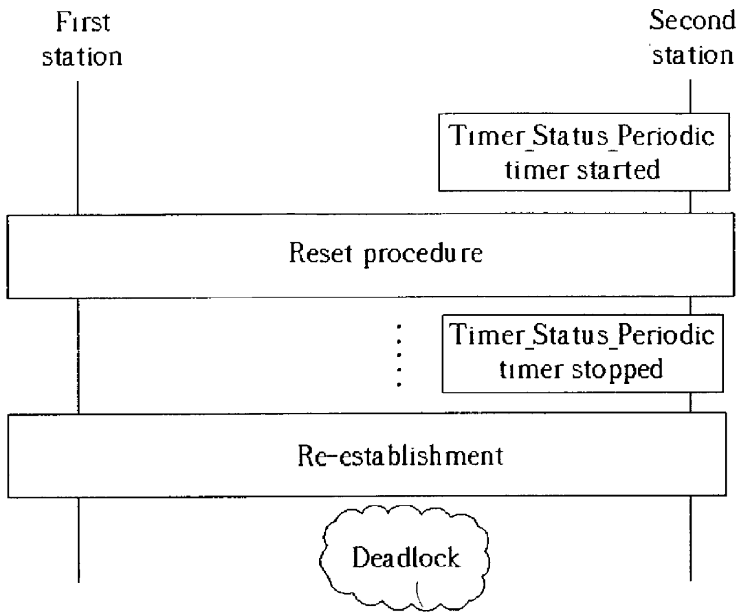
Fig. 5 Prior art
