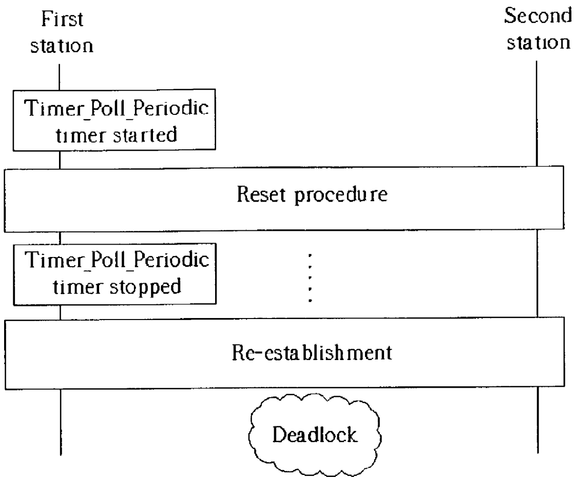
Fig. 4 Prior art
