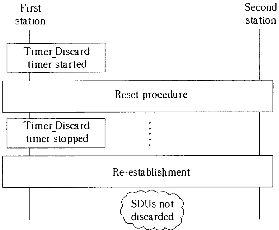
Fig. 6 Prior art
