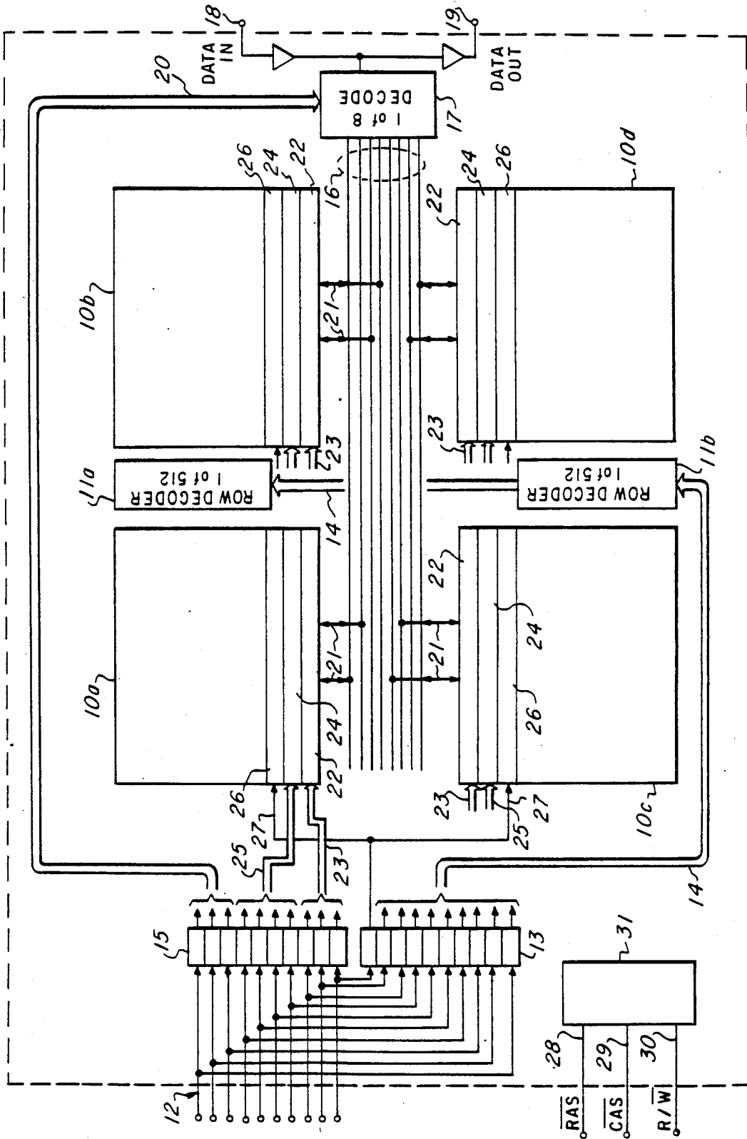
SEMICONDUCTOR CHIP Fig. 1
