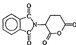
phthaloyl glutamic anhydride (PGA)
