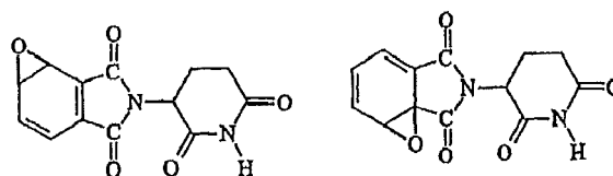
Epoxides of thalidomide
