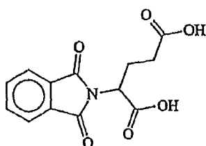
phthaloyl glutamic acid (PG Acid)
