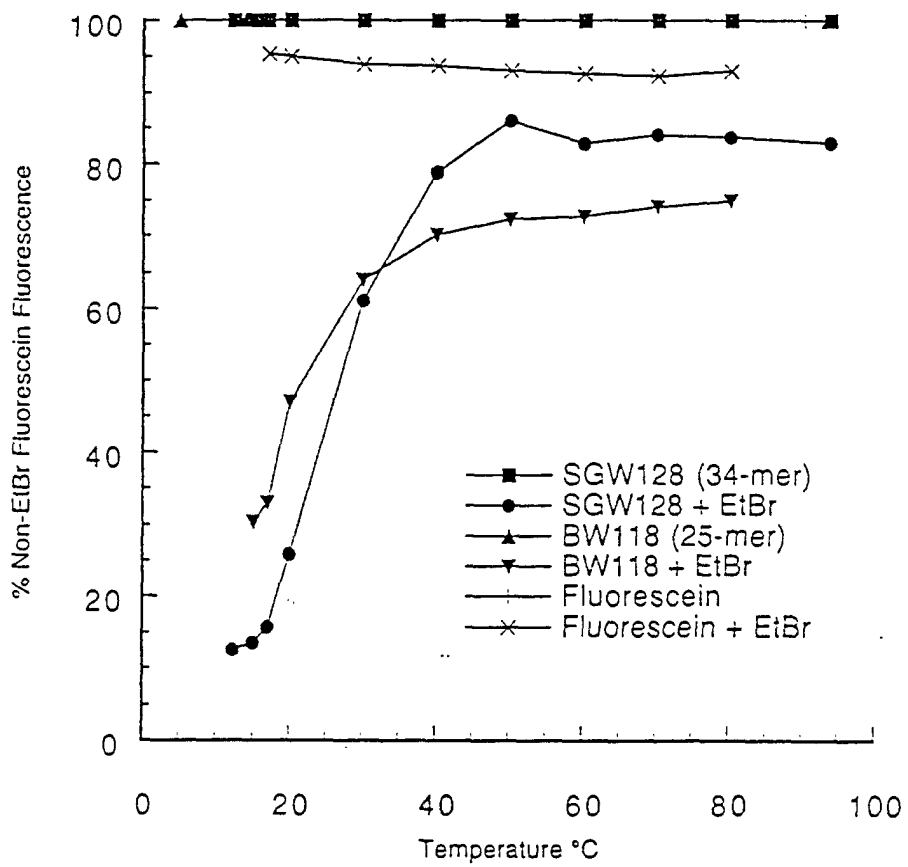
Normalized Fluorescence of 0.5 \mu M Fluorescein & FAM-Labelled Probes \pm 4 \mu g/ml EtBr
