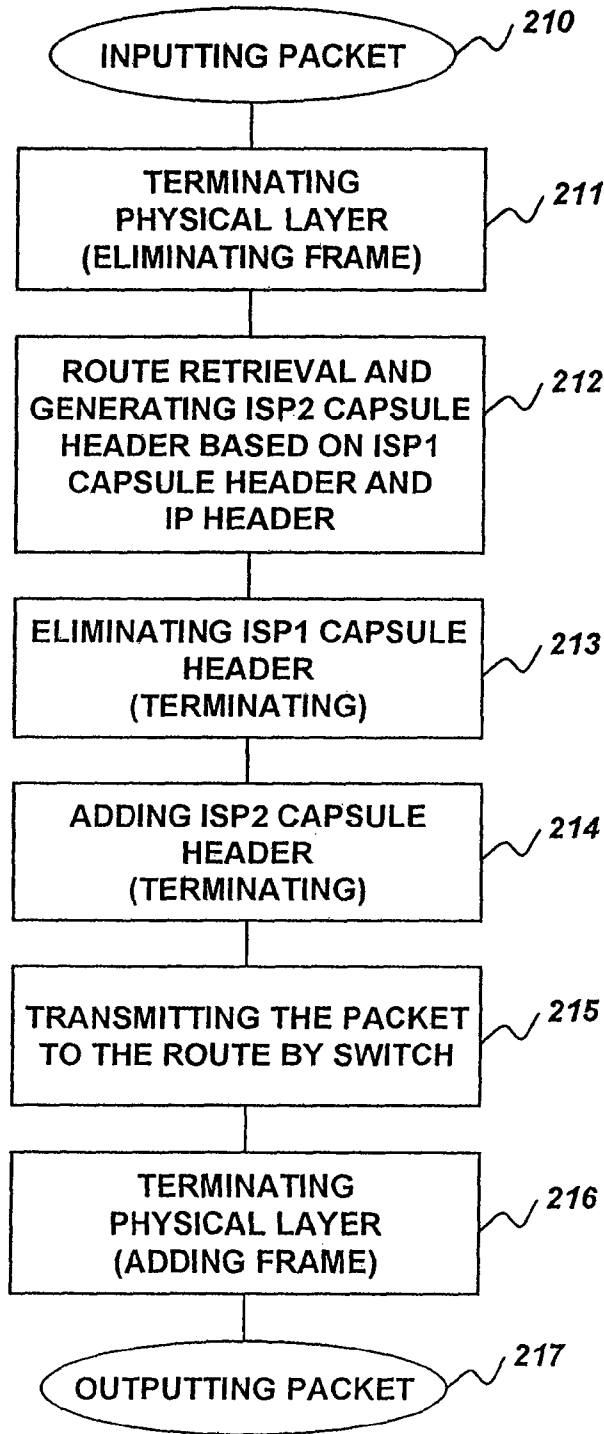
PROCESSING FLOW IN INTERWORK ROUTER
