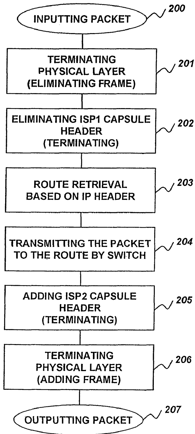
PROCESSING FLOW IN ROUTER
