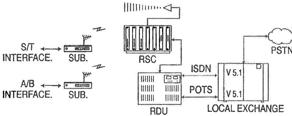
ISDN AND POTS NETWORK INTERFACE
