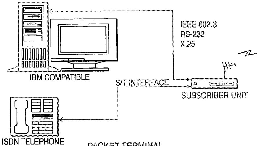
PACKET TERMINAL FIG. 2C
