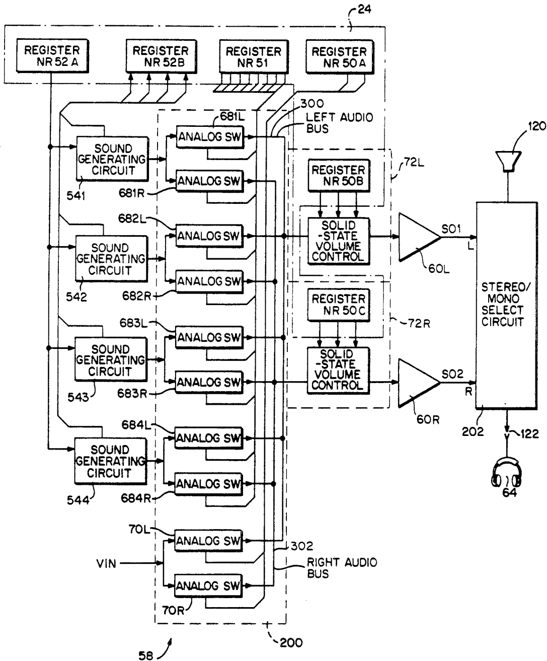
FIG. 4 SOUND GENERATOR
