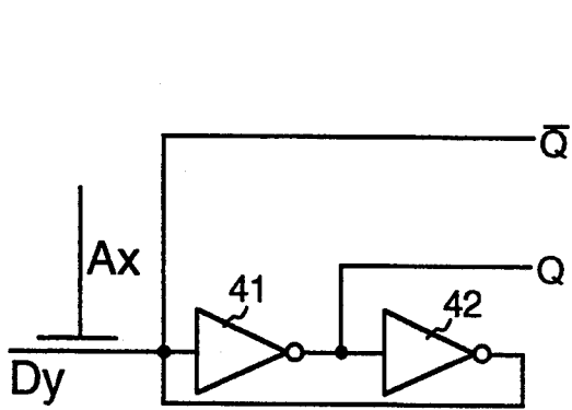
FIG. 4 (PRIOR ART)
