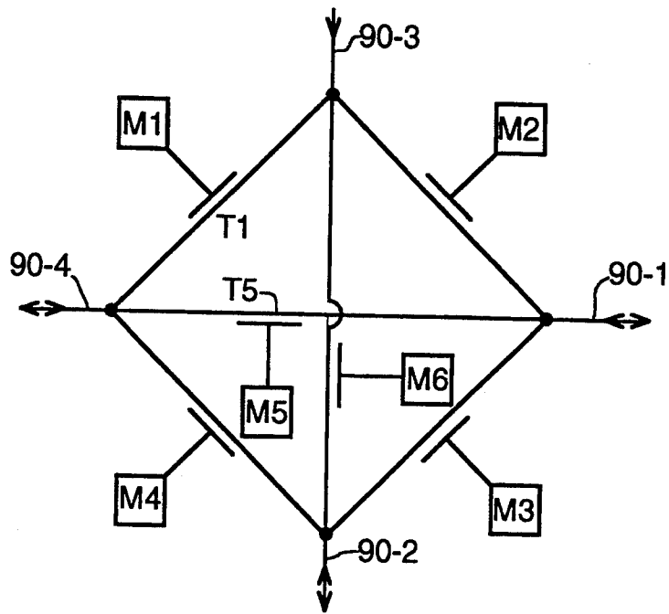
FIG. 2c (PRIOR ART)
