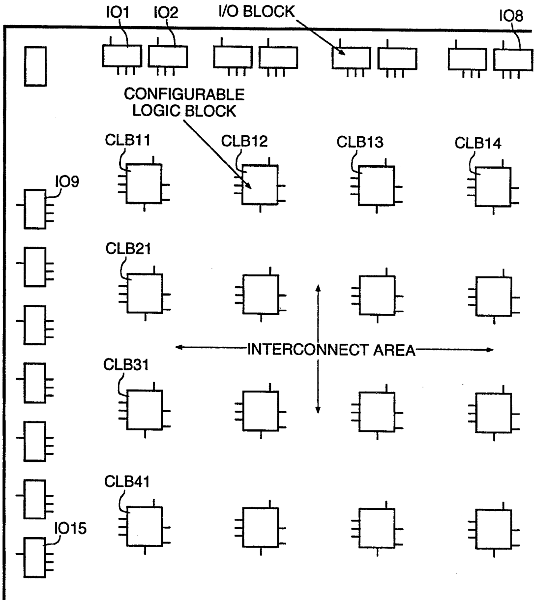
FIG. 1 LOGIC CELL ARRAY STRUCTURE (PRIOR ART)
