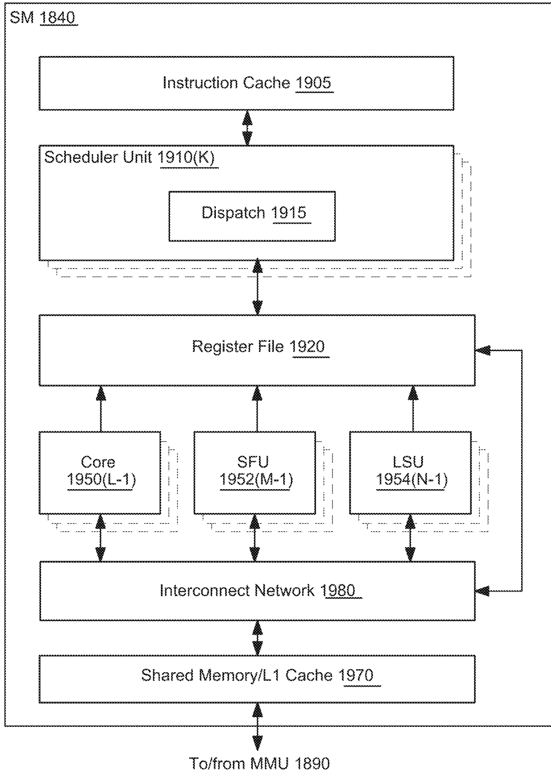
FIG. 23 Example Streaming Multiprocessor
