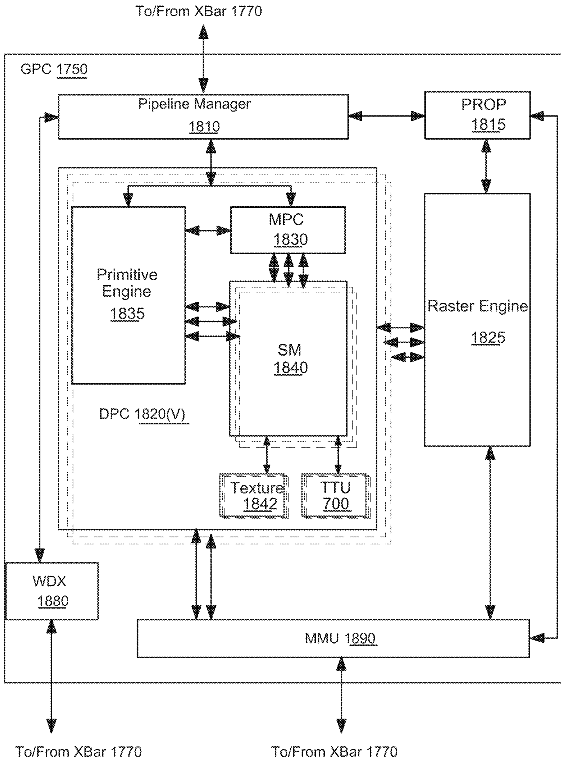
FIG. 21 Example General Processing Cluster
