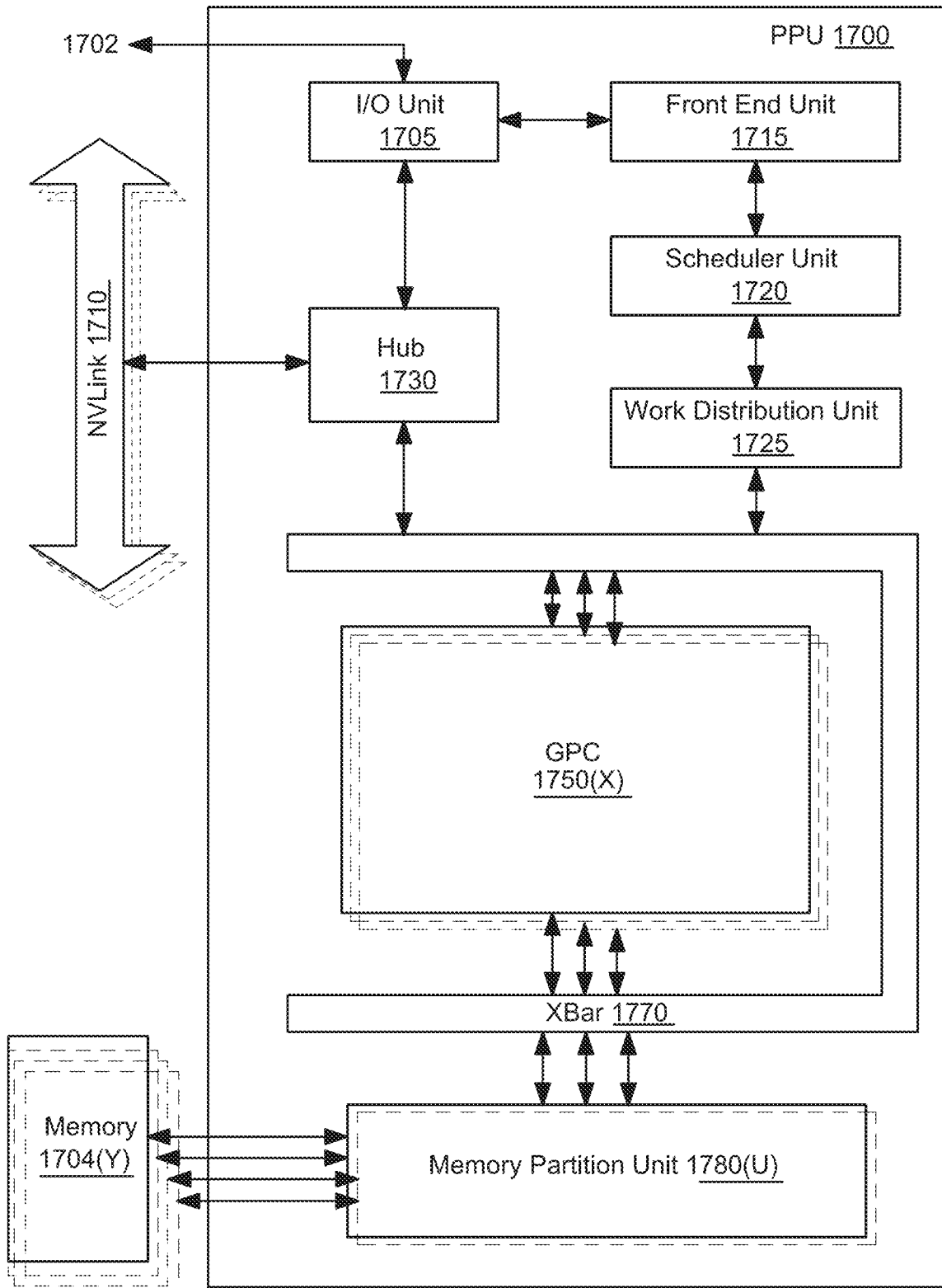
FIG. 19 Example Parallel Processing Unit
