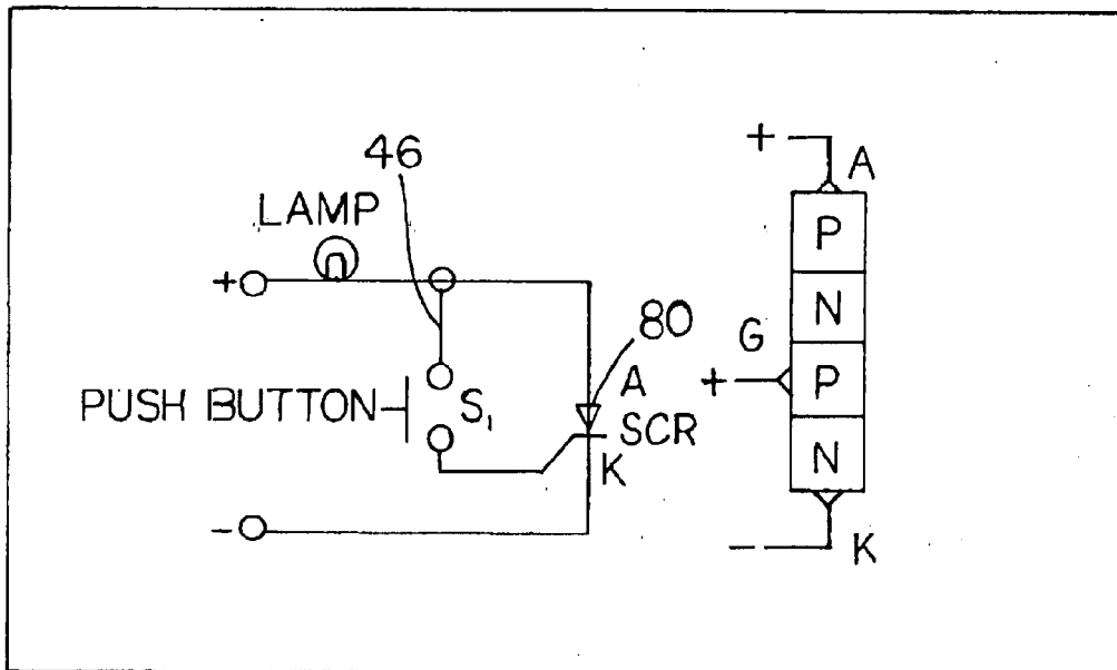
A SIMPLE SCR SWITCHING CIRCUIT
