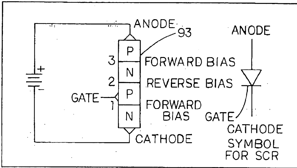
A BLOCK DIAGRAM AND SYMBOL FOR A SILICON CONTROLLED RECTIFIER
