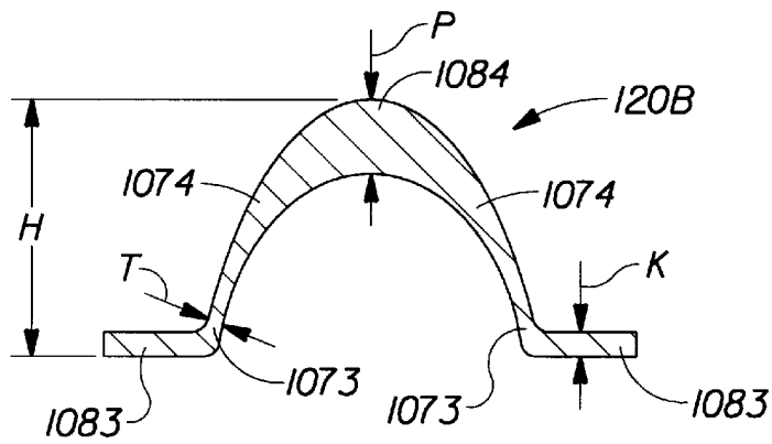
Fig. 8 (PRIOR ART)
