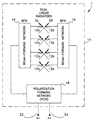
ANTENNA BLOCK DIAGRAM
