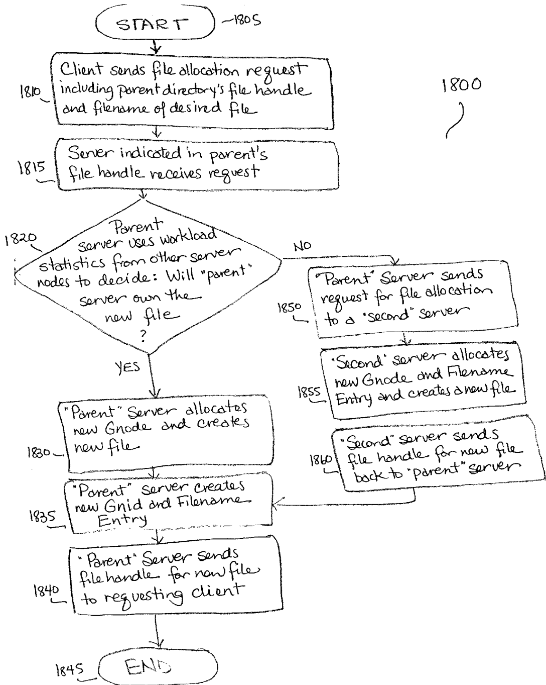
FIGURE 18 - File Allocation
