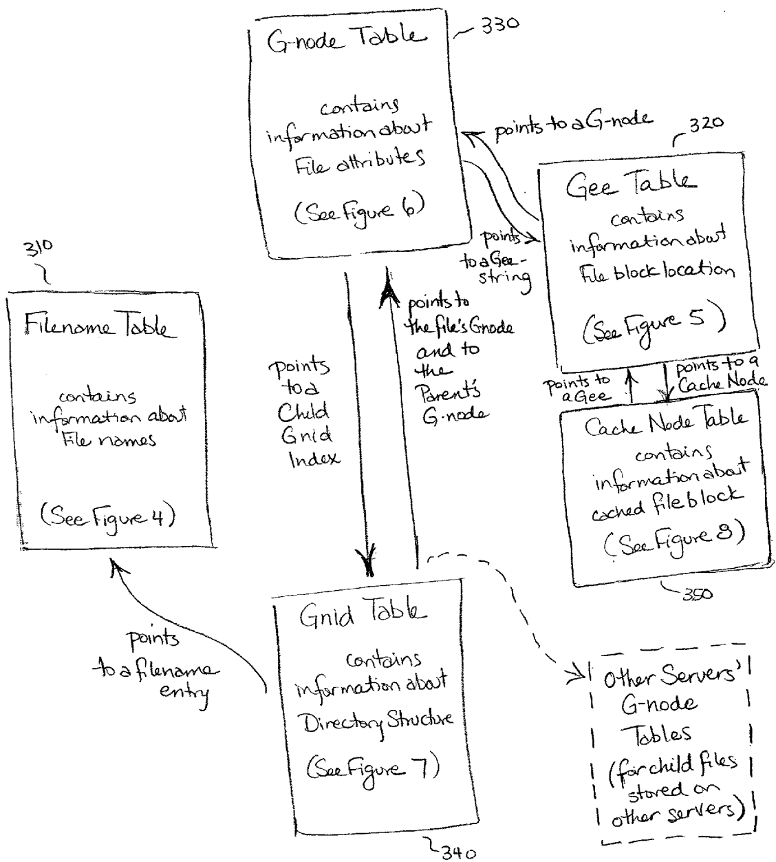
FIGURE 3 - Five metadata structures
