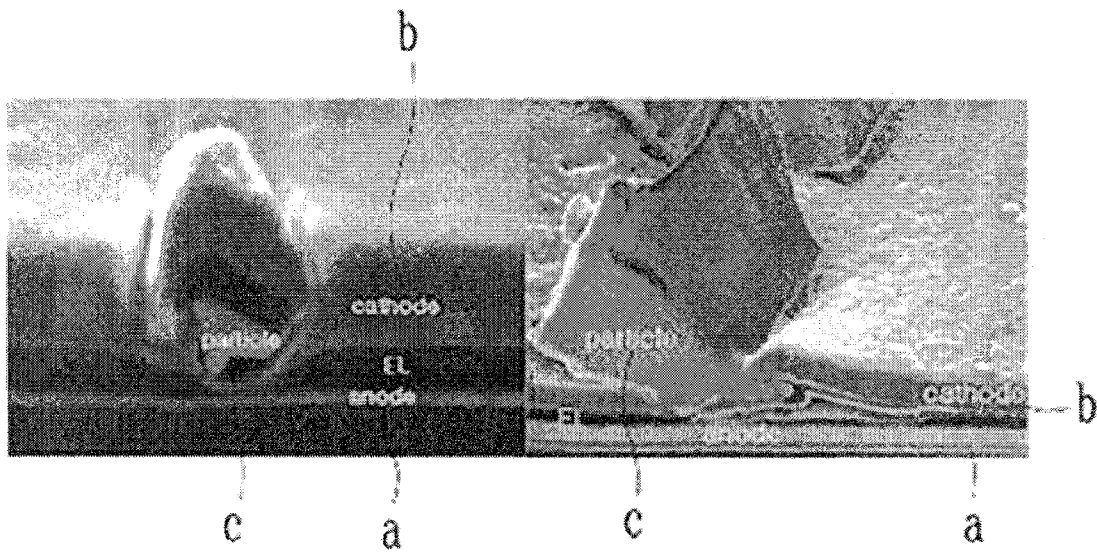
FIG. 4 (PRIOR ART)
