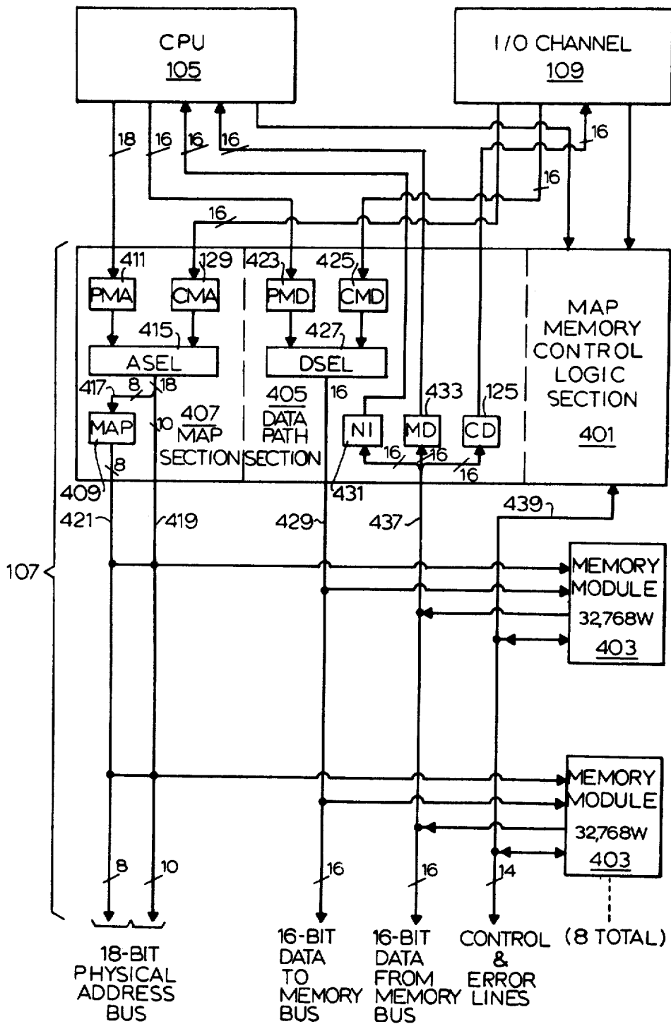
FIG. 34 MEMORY SYSTEM BLOCK DIAGRAM
