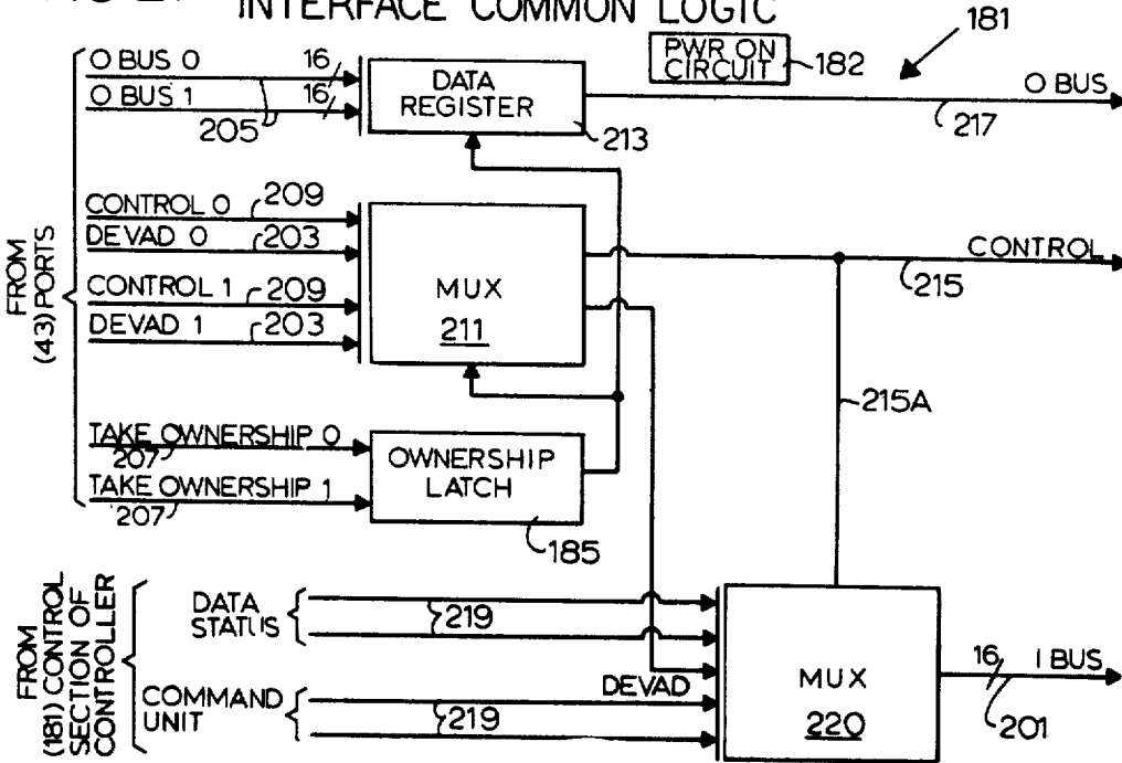
FIG. 21 INTERFACE COMMON LOGIC
