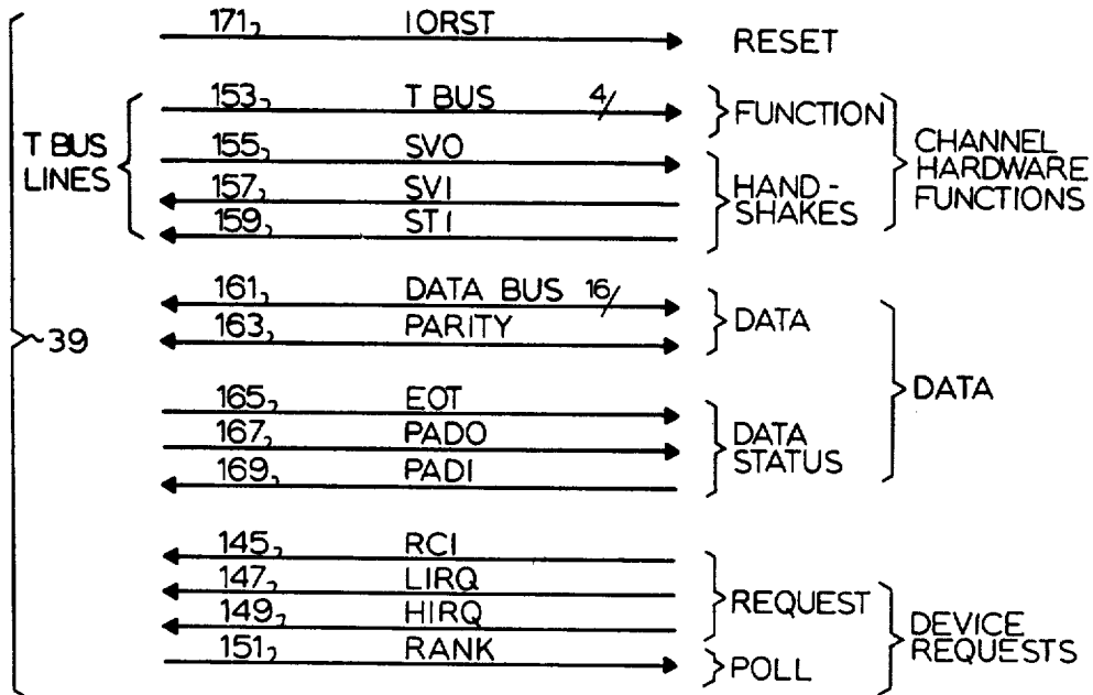
FIG. 14 I/O BUS LINE DESCRIPTION
