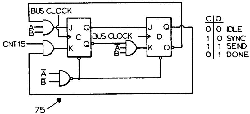
BUS EMPTY STATE LOGIC
