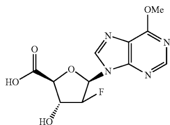
2-deoxy-2-fluoro-5-carboxy- \beta -D-arabinofuranosyl-6-methoxyadenine (5)
