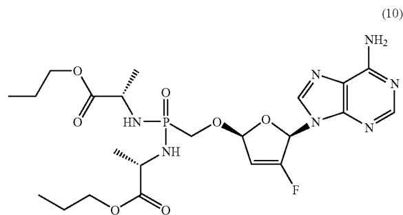
Example of his Amidate Preparation (10)
