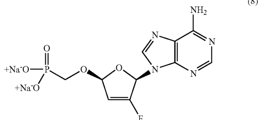
(2'R, 5'R)-9-(3-fluoro-2,5-dihydro-5-phosphonomethoxy-2-furanyl)adenine di sodium salt (8)
