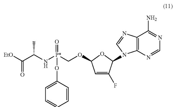
Example of Monoamidate Preparation (11)
