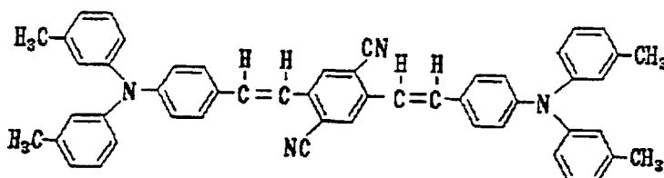
structural formula (3)-6:
