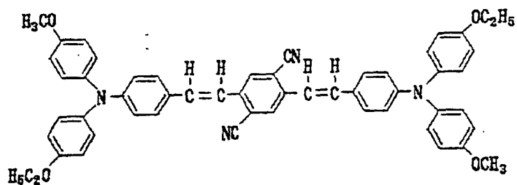
structural formula (3)-2:
