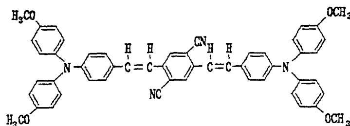
structural formula (3)-1:
