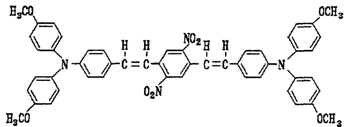
structural formula (3)-5:
