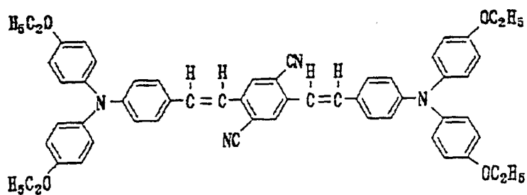
structural formula (3)-3:
