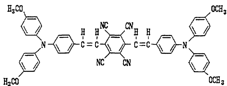
structural formula (3)-4:
