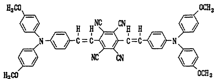
structural formula (3)-4:
