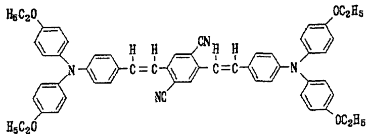
structural formula (3)-3:
