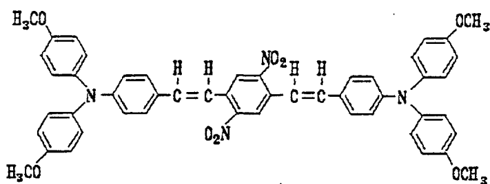
structural formula (3)-5:
