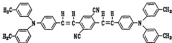
structural formula (3)-6:
