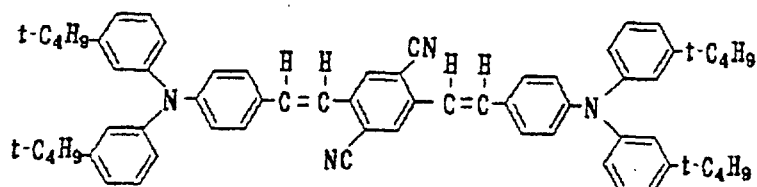
structural formula (3)-7:
