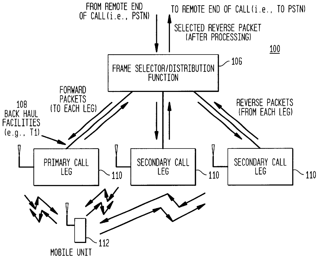
FIG. 2 (PRIOR ART)
