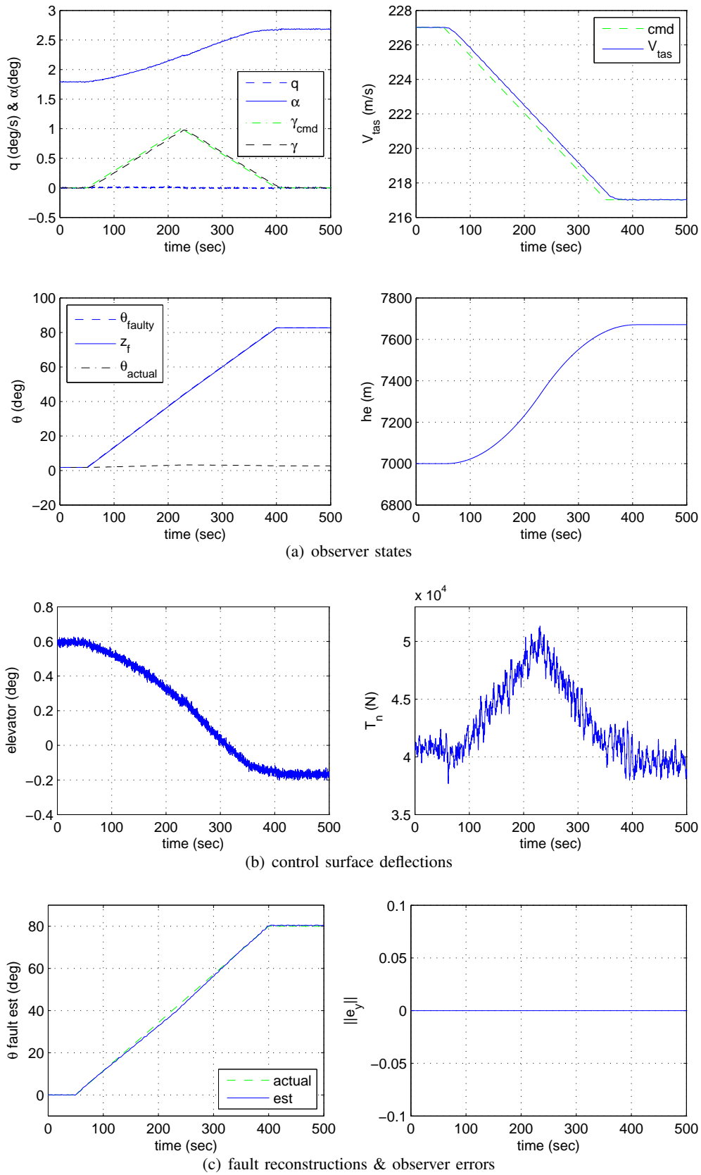
Fig. 2. Nonlinear model simulation: \theta fault
