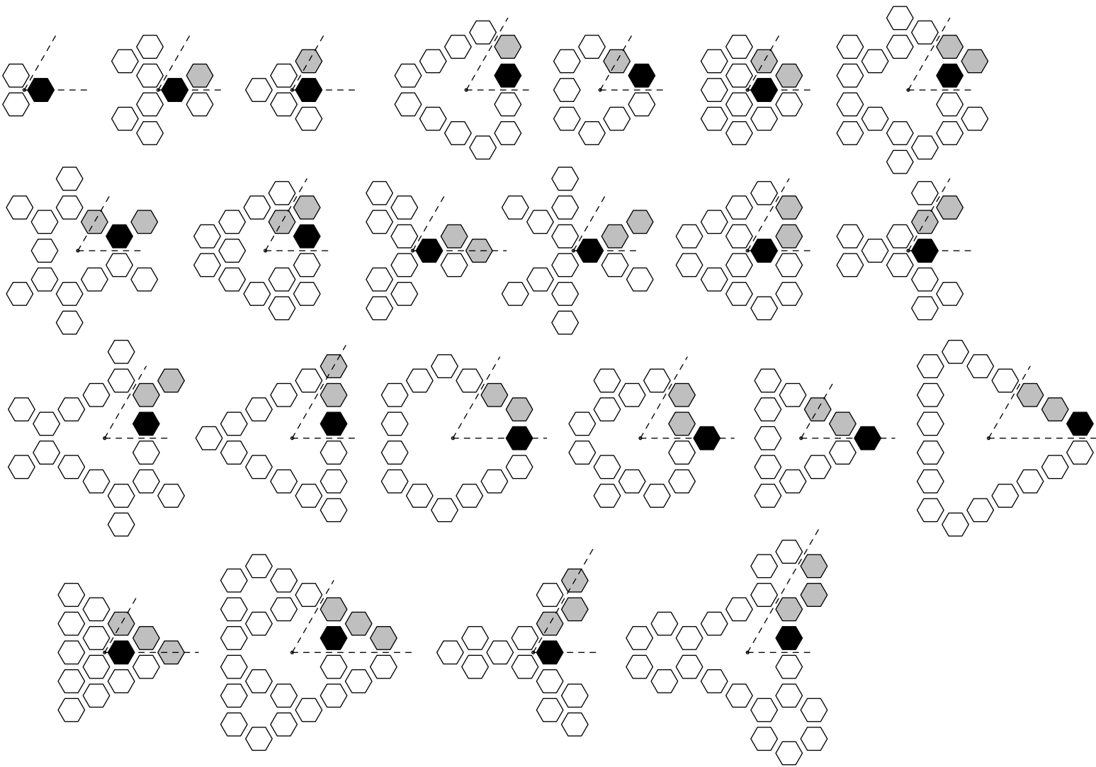
Mapping a \{6, 3\} fixed polyomino to one or two vertex-centered achiral polyominoes with threefold rotational symmetry
