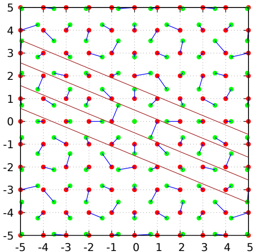
Strip bijection between grids G and H
