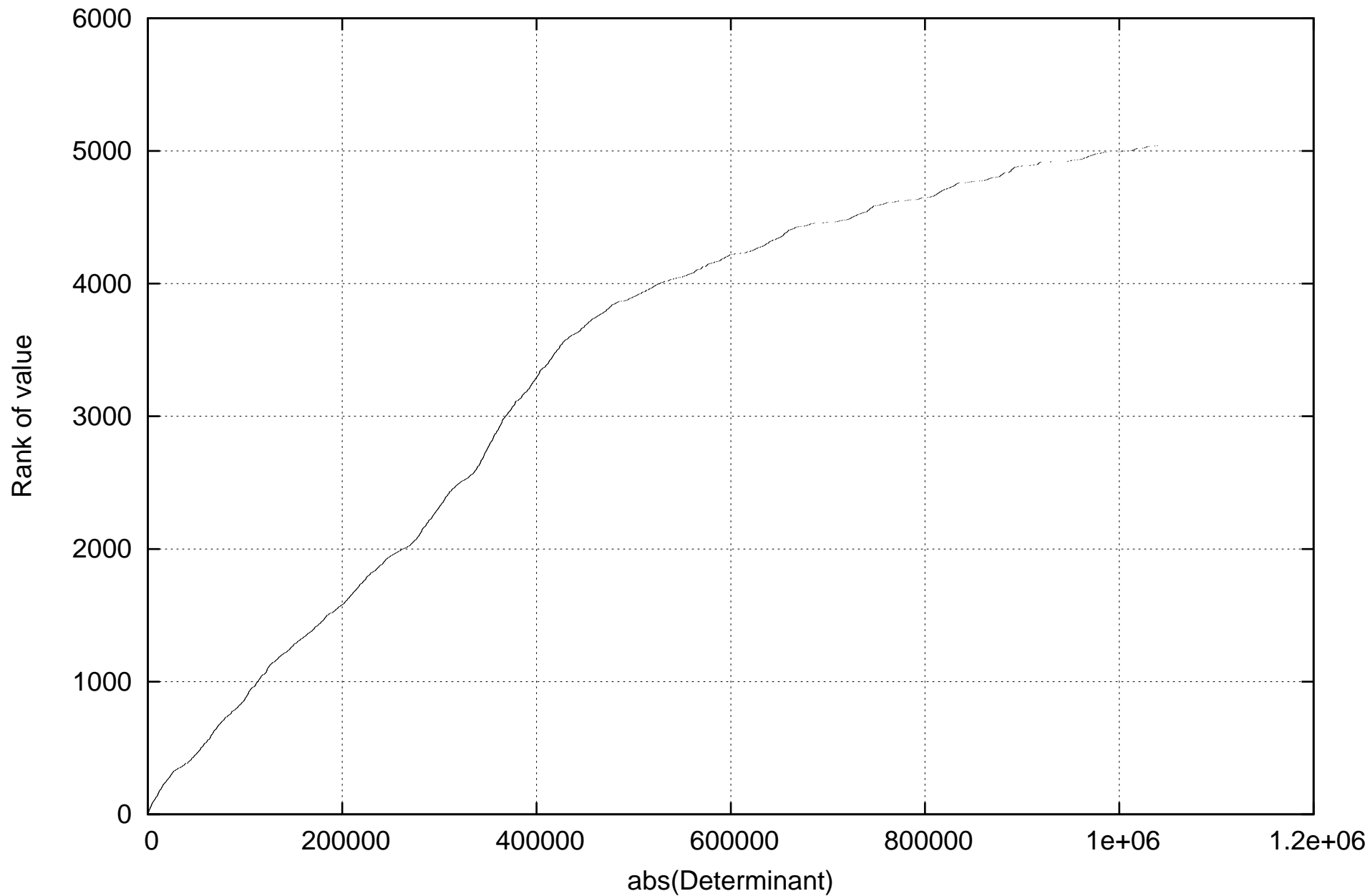
3X3 matrices made from permutations of {99,97,89,87,61,54,20,1,0}
