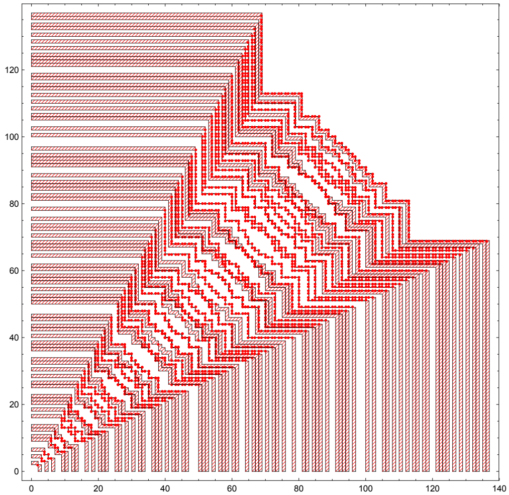
Symmetric representations of \sigma(n) , n \leq 137 , that have two regions of width 1.
