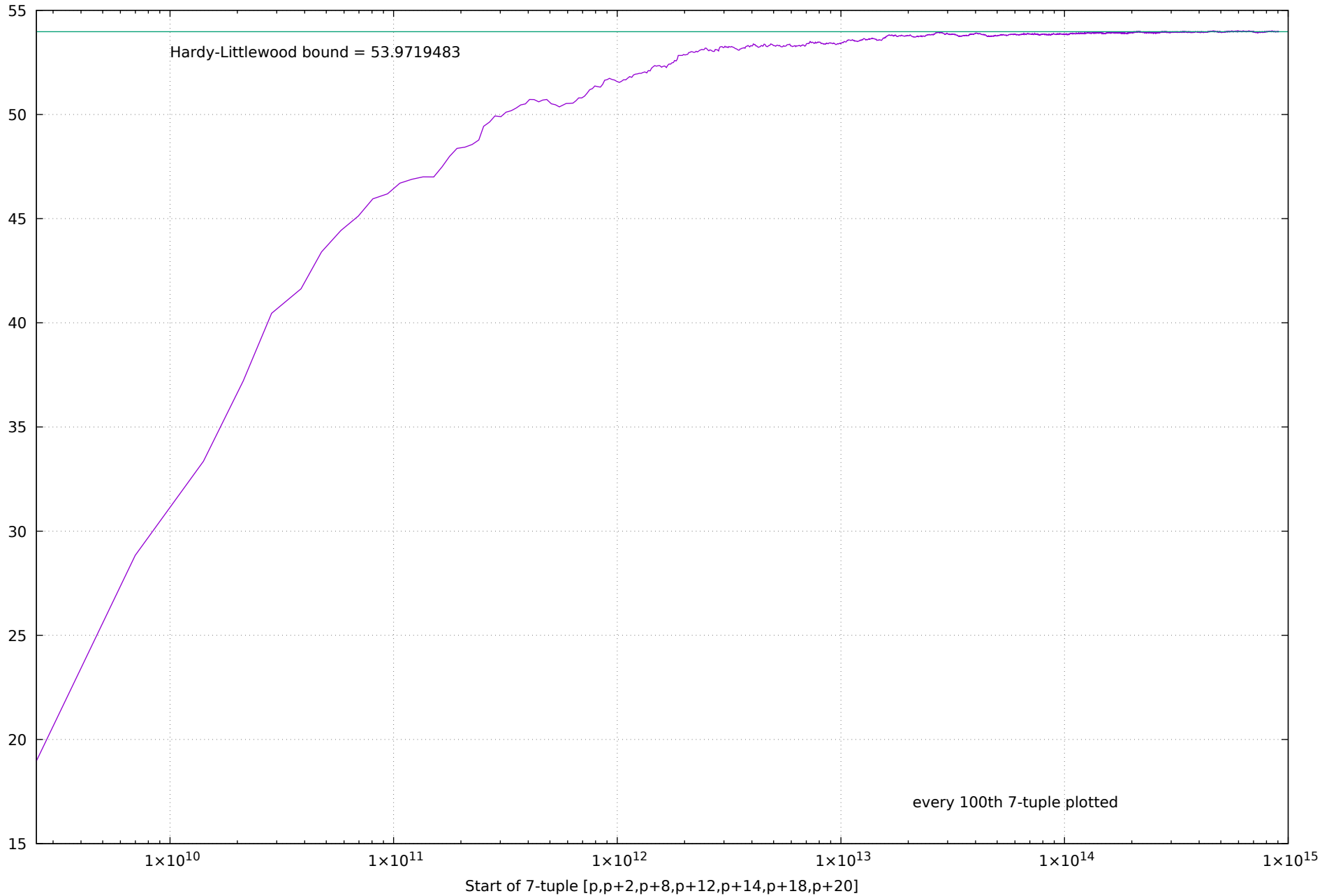
Number of prime 7-tuples / \text{Li}(1/\log(p)^7)
