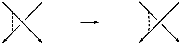
Figure 3.2. Flipping a crossing
