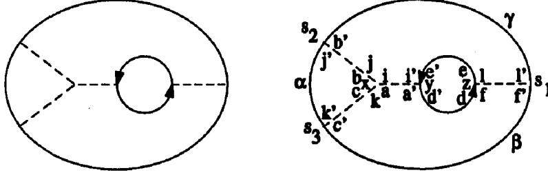
Figure 2.3. An unmarked diagram and its marking.
