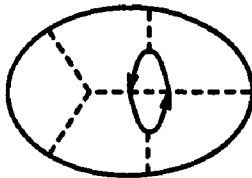
Figure 2.1. An example for a Feynman diagram of order 4, having 5 type X^2A vertices, 2 type \bar{c}Ac vertices, one type A^3 vertex, 5 gauge propagators, and 2 ghost propagators.
