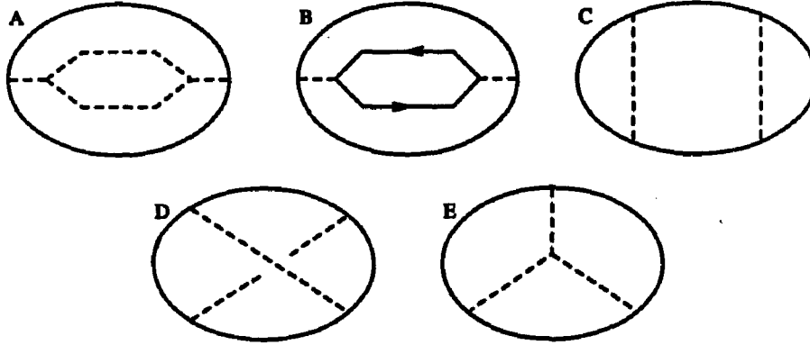
Figure 4.1. The five two-loop diagrams.
