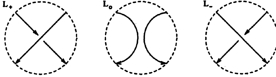
Figure 5.3. The links involved in the skein relation.
