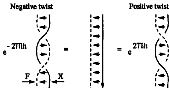
Figure 5.2. The change in \mathcal{W} under a single twist.
