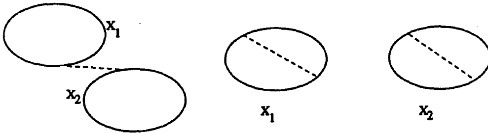
Figure 3.1. First order diagrams
