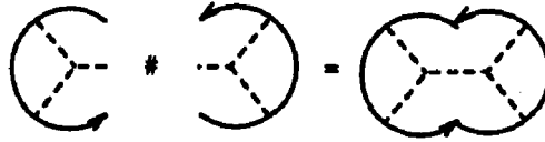
Figure 8.6. Sewing two diagrams.
