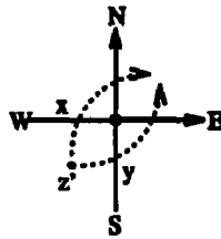
Figure 8.13. The graph SW and the two ways of getting from it to NE . Notice that z' is perpendicular to the plane and therefore appears as a single dot.
