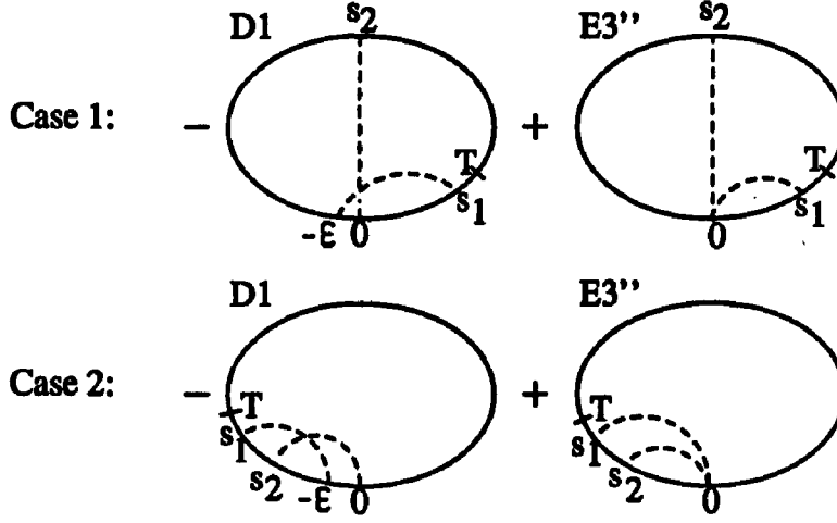
Figure 4.4. The two exceptional cases for D1 \leftrightarrow E3'' .
