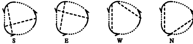
Figure 8.12. The diagrams S , E , W , and N . (The dotted arcs represent parts of the diagrams that are not shown in the figure. These parts are assumed to be the same in the four diagrams)
