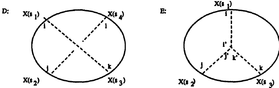
Figure 4.2. The two contributing diagrams.
