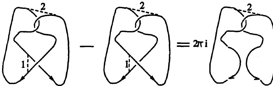
Figure 4.5. The change in \tilde{\mathcal{W}}_2 under a flip.
