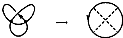
Figure 8.11. The diagram corresponding to a saturated graph with i = 2
