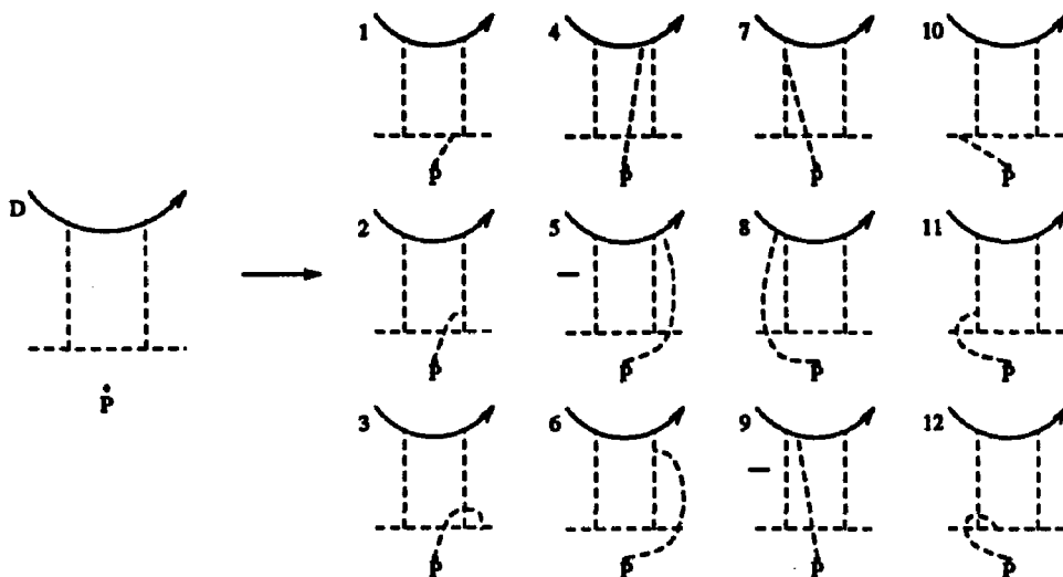
Figure 8.7. A simple invariance proof — the tensor \mathcal{D} is the sum of 1-12. Relation IHX shows that 1 + 2 + 3 = 10 + 11 + 12 = 0 , relation STU shows that 4 + 5 + 6 = 7 + 8 + 9 = 0 , claim 1 shows that 1 + 12 = 2 + 6 = 7 + 11 = 0 , and 4 + 9 = 0 by the choice of signs. It follows that 3 + 5 + 8 + 10 = 0 . This is exactly the fact that \mathcal{T} is an invariant tensor.
