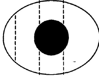
Figure 8.10. An example for a diagram with C'_g(D) = 0
