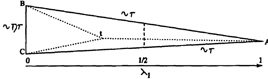
Figure 4.3. The triangle ABC .
