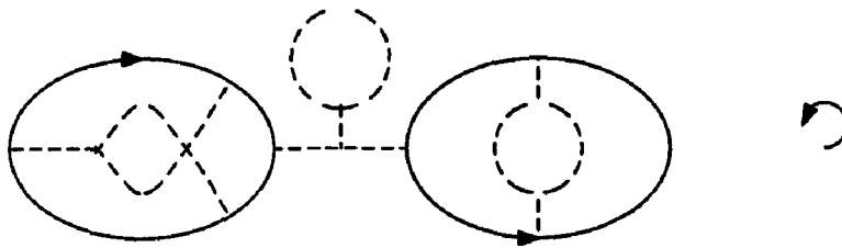
Figure 8.1. An example for a closed diagram of order 6.
