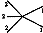
Figure 6.1. The vertex corresponding to the monomial x_1^2 x_2^3 .
