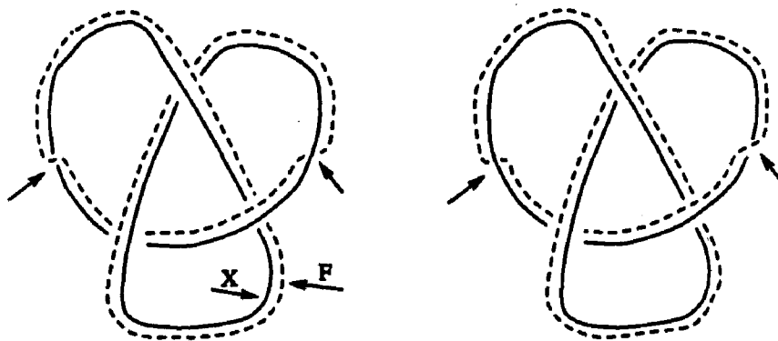
Figure 5.1. A knot with two of its possible framings. (The arrows indicate the differences between the two framings)
