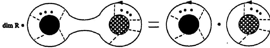
Figure 8.8. The factorization property.
