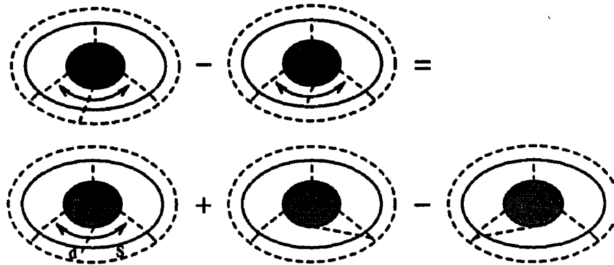
Figure 7.3. The boundary term R1 : In these diagrams, the solid ellipses represent the knot X and the dashed ellipses represent the deformed knot X + \omega . The first two diagrams represent the part of the contribution to \delta \int \mathcal{E}(D) coming from varying the position of one of the X^2A vertices in D . This X^2A vertex is integrated over a range (marked by a double arrow \leftrightarrow ) bounded by two neighboring X^2A vertices. By Stokes' theorem, the quantity that we are interested in, the difference of the first two diagrams, is given by an integral of d^L V on the variation surface S (represented by the third diagram), plus the evaluation of V on the two short segments connecting the solid and the dashed ellipses near the bounding X^2A vertices. This last contribution is given by the term R1 .
