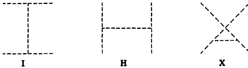
Figure 8.3. The diagrams I , H , and X .
