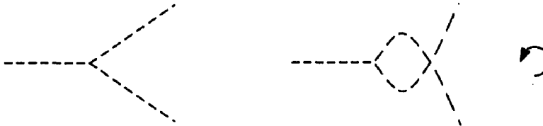
Figure 8.2. Two diagram parts which differ only by the orientation of one of their vertices.
