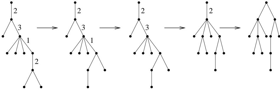
Figure 9: An example of the bijection of item (uuu)
