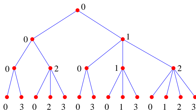
Figure 11: The tree for Exercise 6.19(h 6 )
