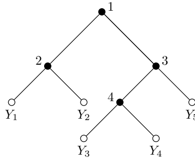
FIGURE 2. A tree in \mathcal{T}_4 of weight (Y_1 + Y_2)Y_1(Y_3 + Y_4)Y_3 .
