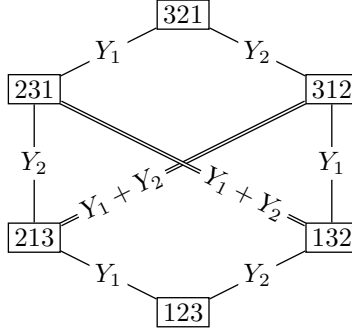
FIGURE 1. The Bruhat order on S_3 marked with the Chevalley multiplicities.
