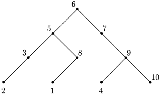
FIG. 5. A local binary search tree.
