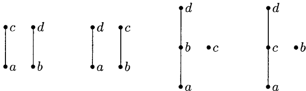
FIG. 6. Obstructions to sleekness.
