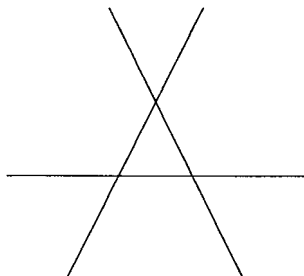
FIG. 2. Seven regions of the Linal arrangement \mathcal{L}_2 .
