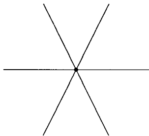
FIG. 1. The Coxeter hyperplane arrangement \mathcal{A}_2 .
