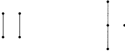
FIG. 3. Forbidden subsets for semiorders.
