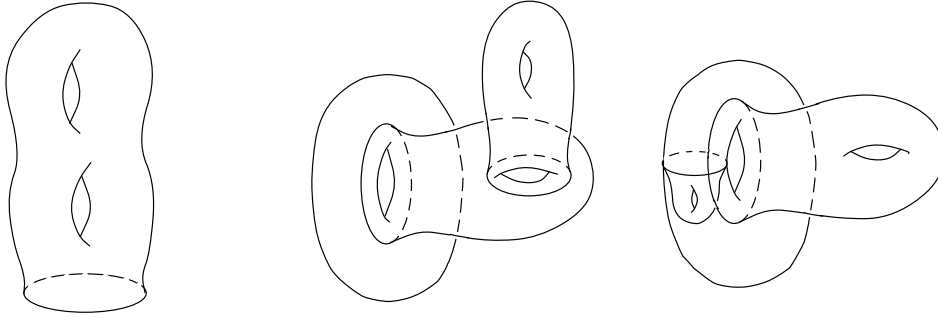
Figure 1: A grope of class 2 is a surface – two closed gropes of class 4
