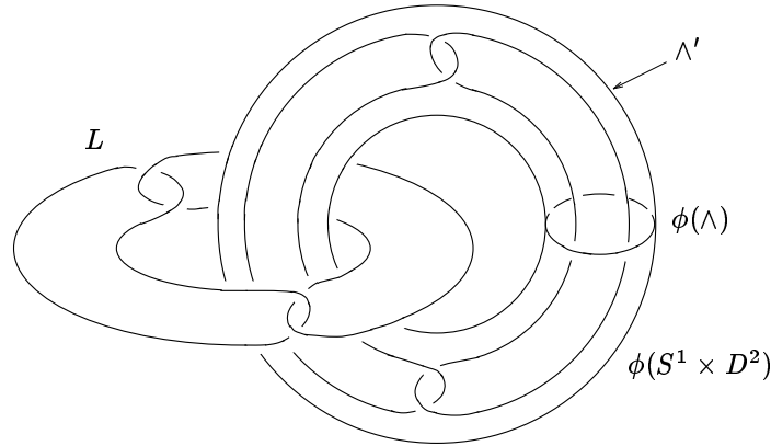
Figure 7: In this example \widehat{L} is the Borromean rings, and Q is the Bing double of the core circle of S^1 \times D^2 .
