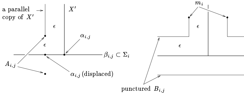
Figure 5: Steps 1 and 2 at a distance \epsilon from X
