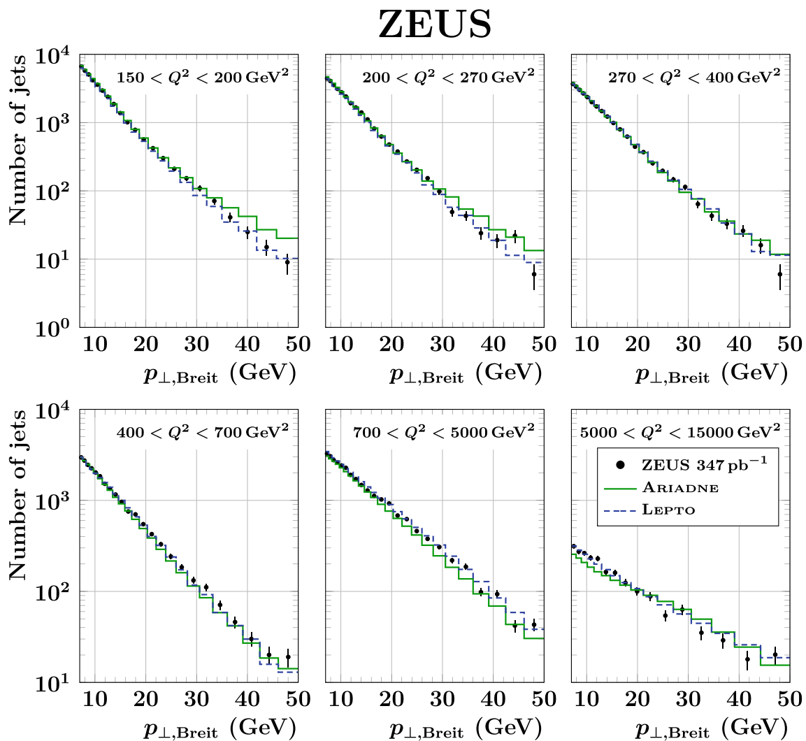
Fig. 2 Detector-level comparison of data (dots) and the ARIADNE (solid, green) and LEPTO (dashed, blue) MC distributions after corrections for the p_{\perp,Breit} distribution in different regions of Q^2 . The data are shown after subtracting the background from photoproduction and low-
