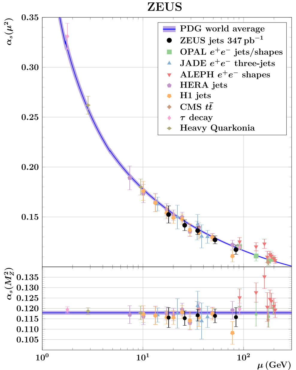
Fig. 10 Value of the strong coupling \alpha_s(\mu^2) as a function of the scale \mu . The data points indicate determinations from measurements that were performed close to the indicated scale. The uncertainties represent the full uncertainty of each determination. All depicted results were obtained at least at NNLO. They are based on data from e^+e^- [63–65], ep [54,66] and pp [67] collisions, as well as from \tau lepton decays [68] and quarkonium states [69]. The solid blue line shows the PDG world average [61]. Also shown are the \alpha_s(M_Z^2) values corresponding to each data point
