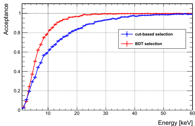
Fig. 10 Acceptance vs energy for the cut-based analysis and the multivariate BDT analysis
